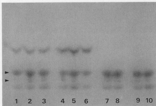
Fig. 1. The Ldh of mouse blood. Lanes 1 to 6: infected mice. Lanes 7 to 10: control mice. Migration goes from bottom to top. Bands with \blacktriangleright are due to hemoglobin. The lower band is mouse Ldh , the upper band is parasite Plasmodium yoelii yoelii Ldh .
