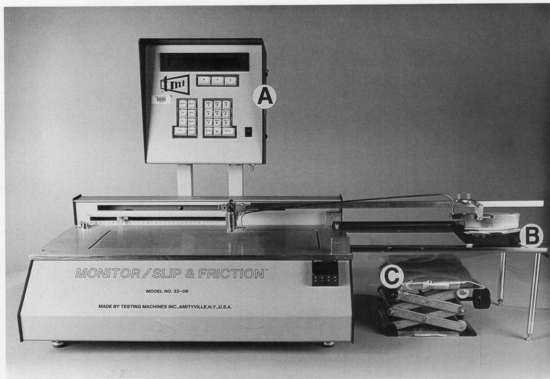
Fig. 1. Frontal view of the slip and friction tester machine showing the liquid crystal display screen and key panel (A), the sled (B), and the adjustable plate (C) to keep the arm secured underneath the sled.
