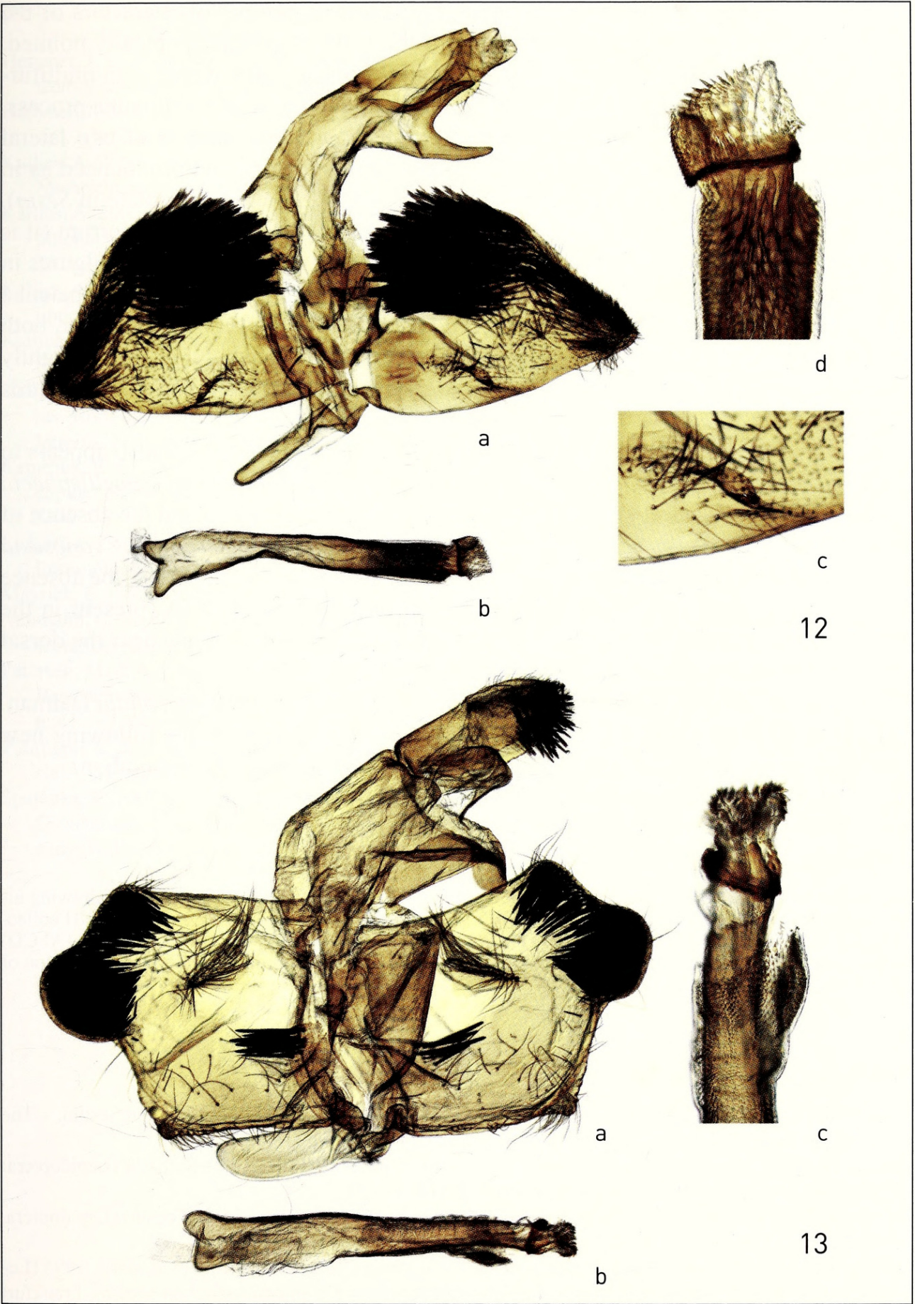
Figs 12–13. Sesiini, male genitalia. 12. Eusphencia melanocephala comb. n. (a) ventral view, (b) phallus, (c) crista of valva, enlarged, (d) distal end of phallus, enlarged. 13. Sesia yezoensis . (a) ventral view, (b) phallus, (c) distal end of phallus, enlarged.
