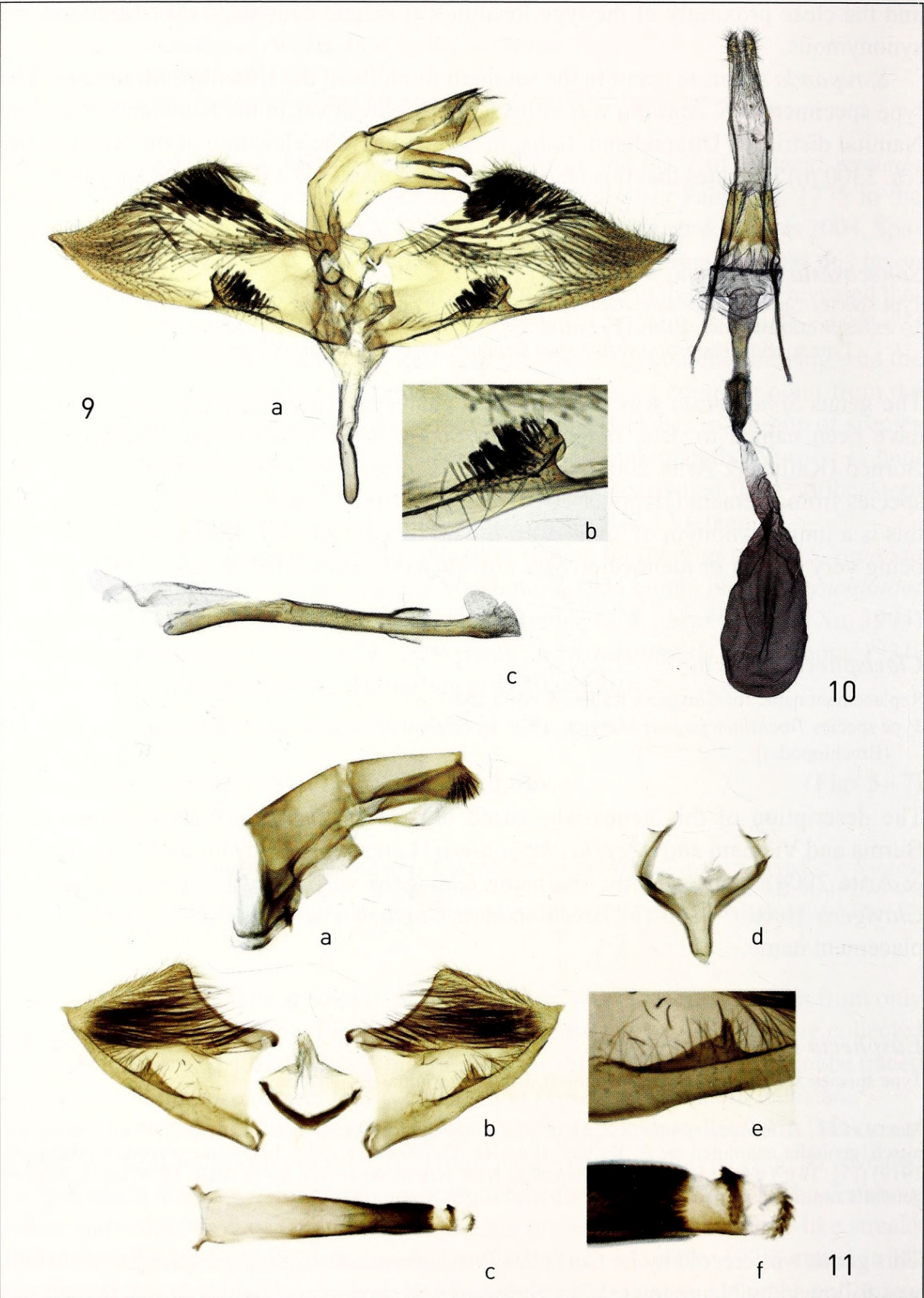
Figs 9–11. Sesiini, genitalia. 9–10. Cyanosesia ormosiae sp. n. 9. ♂, paratype. (a) ventral view, (b) crista of valva, enlarged, (c) phallus. 10. ♀, paratype. 11. Lamellisphesia xerampelina sp. n., ♂, holotype. (a) uncus tegumen complex, (b) valvae and juxta, (c) phallus, (d) vinculum and saccus, (e) crista of valva, enlarged, (f) distal end of phallus, enlarged.
