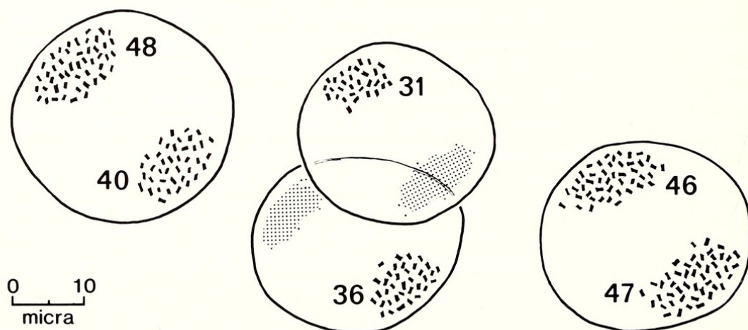
FIG. 1. Anaphase I configurations of pollen mother cells from plants of the intergrading population from Pasto, Colombia (culture 13033).
