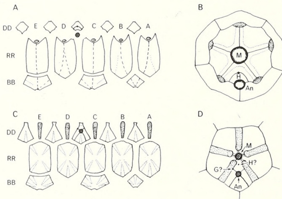
TEXT-FIG. 5. Plate diagrams in coronates and Lysocystites . A, B, Coronates. A, lateral view (broken lines indicate V and W ridges, dotted lines additional lateral ridges found in Stephanocrinus , Tormoblastus , and Paracystis ); B, oral surface. C, D, Lysocystites . C, lateral view (dotted lines indicate outlines of triradiate thecal pore structures); D, oral surface. A-E, Carpenter radii; An, anus; BB, basal plates; DD, deltoid plates; G, gonopore; H, hydropore; M, mouth; RR, radial plates; supposed homologues of blastoid lancet plates stippled. Note that these plates bear the facets for erect arms and always lie in a radial position between a radial plate and two deltoids. Note also that the mouth frame is composed of five deltoids even in Lysocystites where they are elongate.
