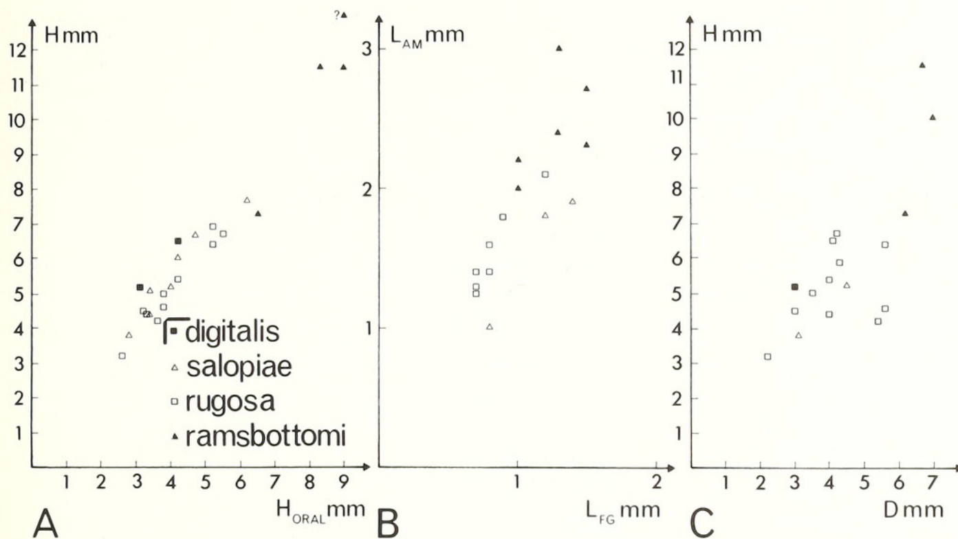
TEXT-FIG. 2. Bivariate plots of some of the measurements shown in text-fig. 1. A, height against height of oral surface. B, length of ambulacrum against length of food groove. C, height against diameter.
