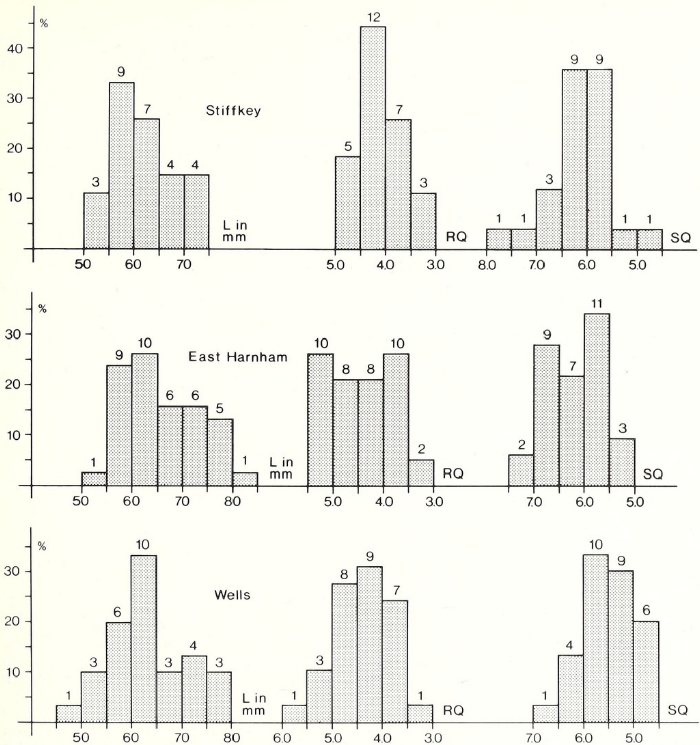
TEXT-FIG. 8. Histograms of the length of the guard (L), Riedel Quotient (RQ), and Slenderness Quotient (SQ) of three samples of Gonioteuthis quadrata quadrata from Stiffkey, East Harnham, and Wells. The figures above the bars are the actual number of specimens.
