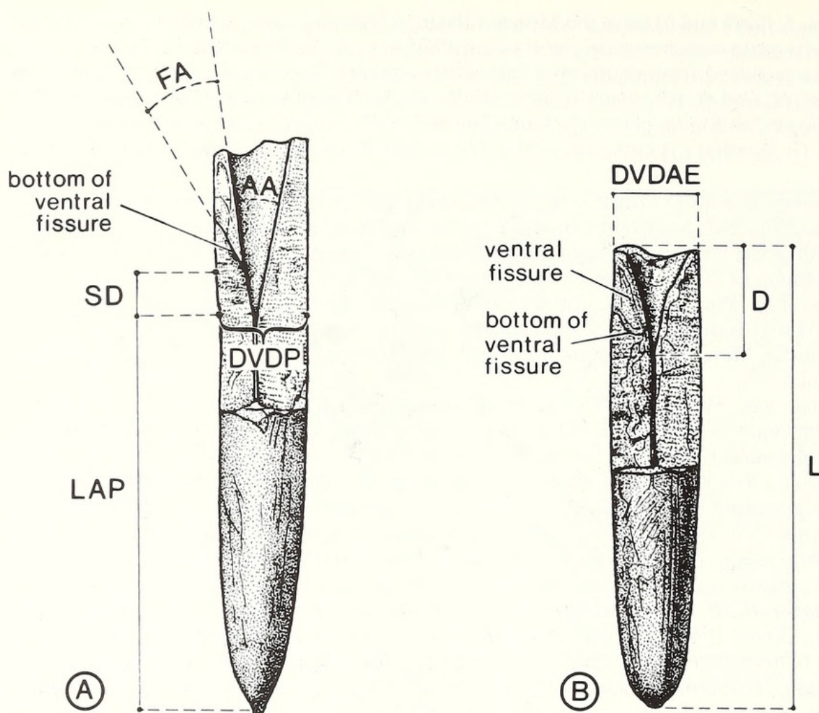
TEXT-FIG. 6. Diagram showing the morphological elements of the guard in (A) Belemnitella praecursor and (B) Gonioteuthis quadrata . L = length of the guard; LAP = length from the apex to the protoconch; D = depth of the pseudoalveolus; SD = Schatzky distance; DVDP = dorso-ventral diameter at the protoconch; DVDAE = dorso-ventral diameter at the alveolar end; FA = fissure angle; and AA = alveolar angle. After Christensen and Schmid (1987).
