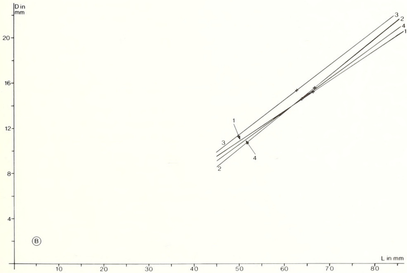
TEXT-FIG. 13. Regression lines of four samples of Goniatites quadrata quadrata . A, length of the guard (L) vs dorso-ventral diameter at the alveolar end (DVDAE). B, length of the guard (L) vs depth of the pseudoalveolus (D). + = mean values. 1, East Harnham; 2, Shawford; 3, Stiffkey; 4, Wells.
