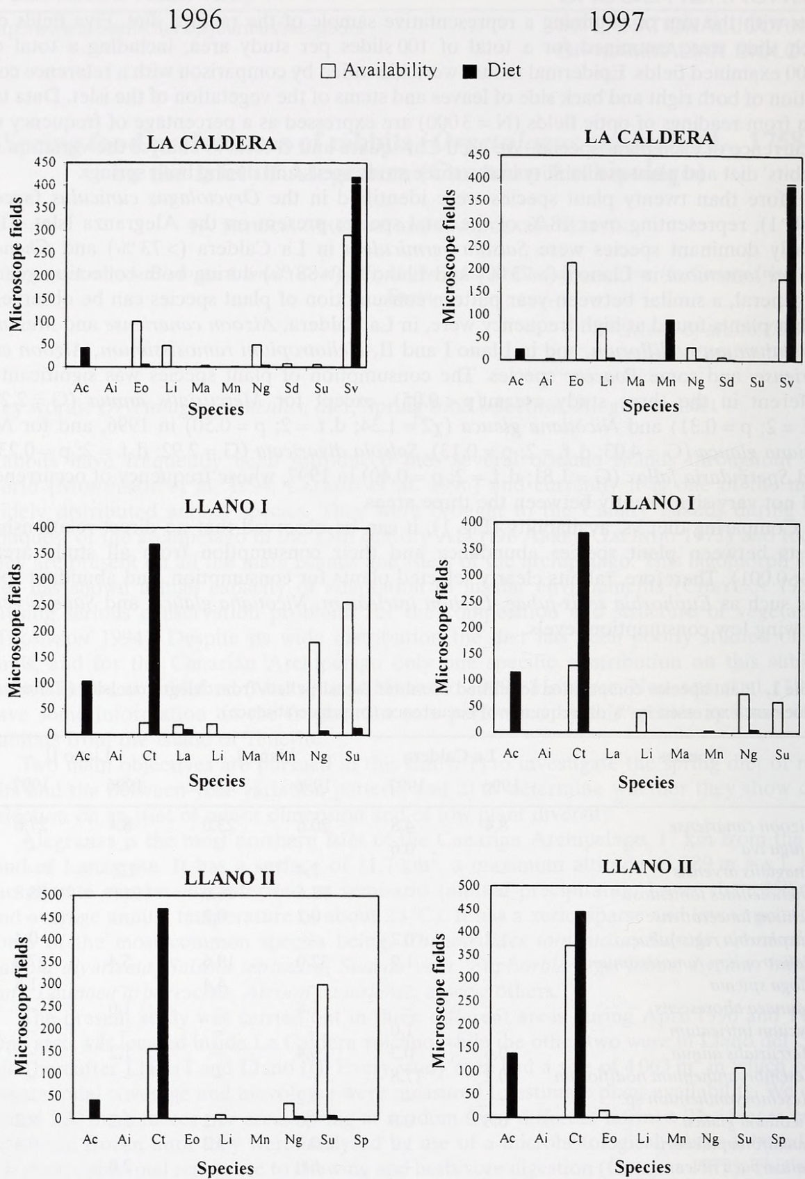
Fig. 1. Comparison between plant availability and diet in the spring of 1996 and 1997 on the Alegranza Islet (Canaries). Data from plant availability were transformed to the same units of optic fields with the aim of relating them to the diet. Ac: Aizoon canariense , Ai: Ajuga iva , Ct: Chenoleoides tomentosa , Eo: Euphorbia regis-jubae , La: Launaea arborescens , Li: Lycium intricatum , Ma: Mercurialis annua , Mn: Mesembryanthemum nodiflorum , Ng: Nicotiana glauca , Sd: Salsola divaricata , Sp: Spergularia fallax , Su: Suaeda vera , Sv: Salsola vermiculata . Only the species present in the study areas were included.
