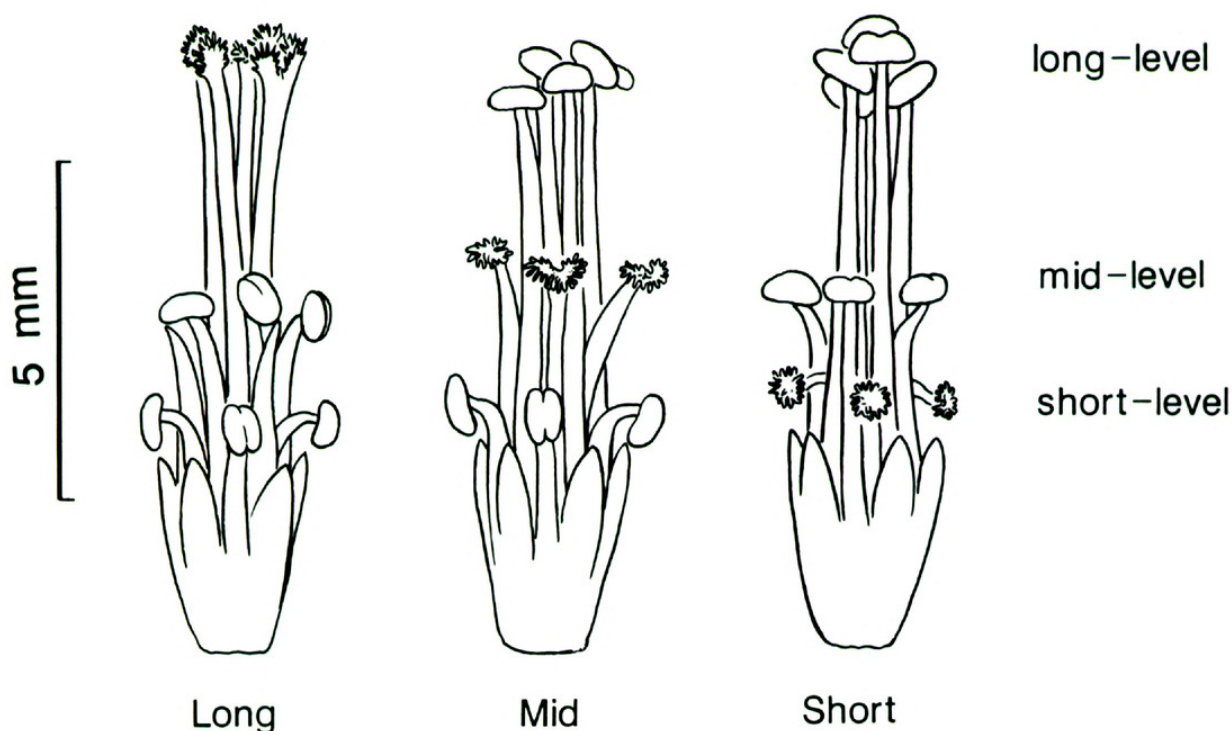
FIGURE 1. Illustrations of gynoecia and androecia of the three floral forms of Oxalis pes-caprae . The designation of each floral form is given below each illustration. The stigma and anther level designations used in the text are given to the right of the figure.
