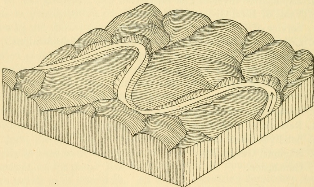
FIG. 1. A meandering valley with narrow flood-plain scrolls.
