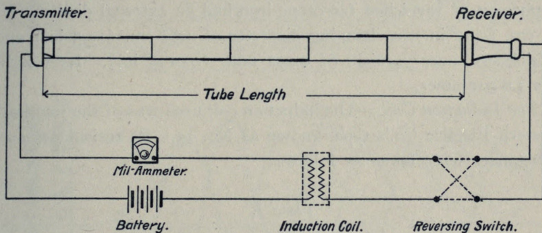
FIG. 1. Diagram of Humming Telephone Connections.
