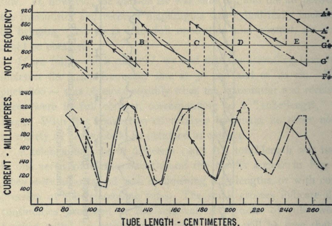
FIG. 5. Effect of Lengthening and Shortening the Tube.
