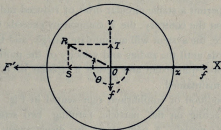
FIG. 16. Vector Diagram of Reinforced Vibration.
