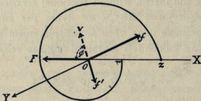
FIG. 15. Vector Diagram of Free Damped Vibration.
