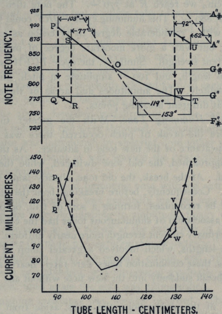
FIG. 6. Humming Cycles with Cyclic Changes in Tube-length.
