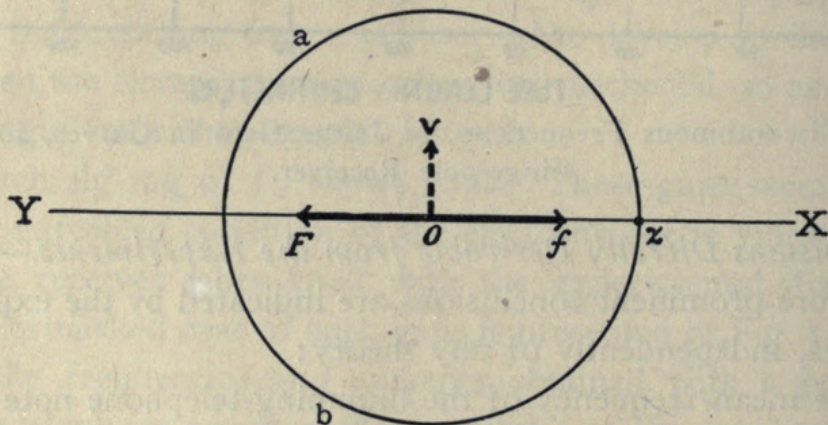
FIG. 14. Vector Diagram of Free Undamped Vibration.
