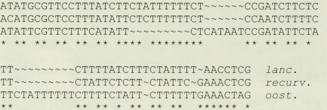
Figure 2. DNA sequences: Trillium lancifolium , T. recurvatum and T. oostingii (top to bottom). Sequence is based on the psbA-trnH intergenic spacer, a non-coding cp gene region (Farmer, 2007).
