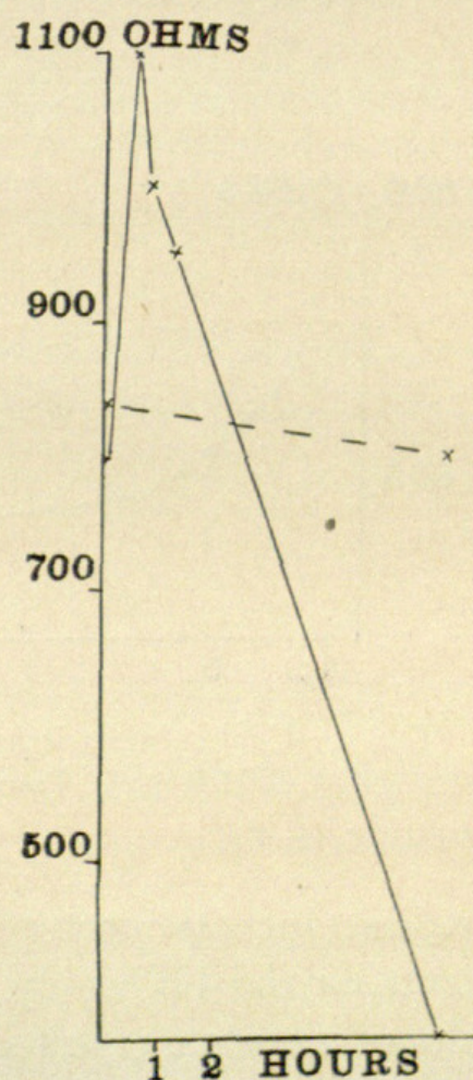
FIG. 6.—Curves of electrical resistance of Laminaria saccharina in sea water 1000 cc. + \text{Al}_2(\text{SO}_4)_3 \cdot 18 \text{H}_2\text{O} 6.7 gm. ( =0.01 \text{ M} ) (unbroken line), and of a control in sea water (dotted line).
