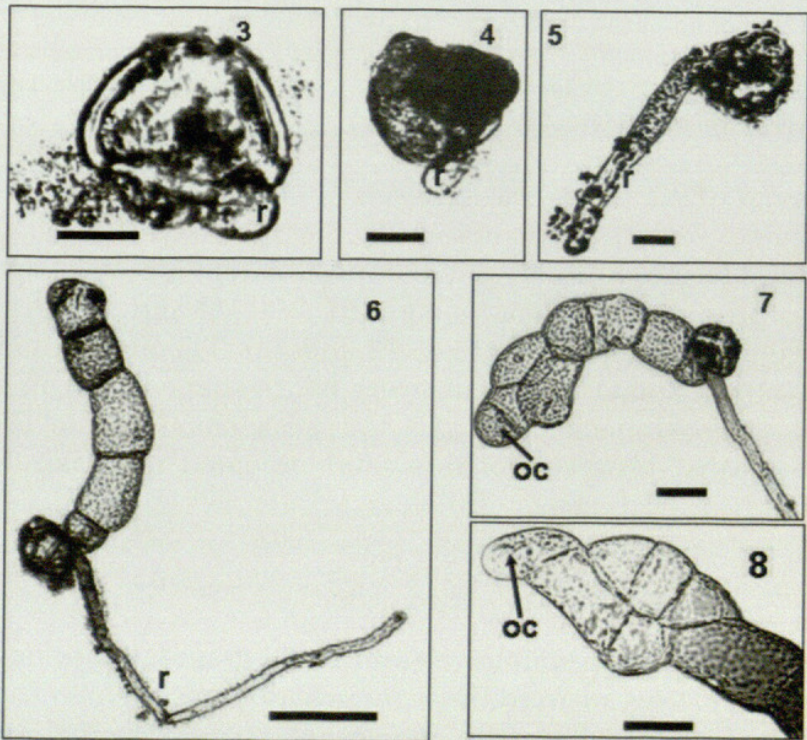
FIGS. 3–8. Initial phase of spore germination. Bars = 20 \mu m. 6. Germinated spore with rhizoid. Bar = 20 \mu m. 7. Filamentous gametophyte (15 days). Bar = 100 \mu m. 8–9. Laminar gametophyte with the initial lateral divisions (15 days). Bars = 50 \mu m. Legend: oc – obconic cell, r – rhizoid.
