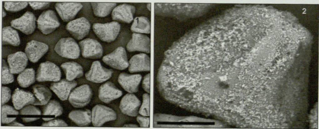
FIGS. 1–2. 1. Scanning electron micrographs of Dicksonia sellowiana spores. 2. Tetrahedral spores. Bar = 100 \mu m. 3. Detail of the spore with densely granulated surface. Bar = 20 \mu m.
