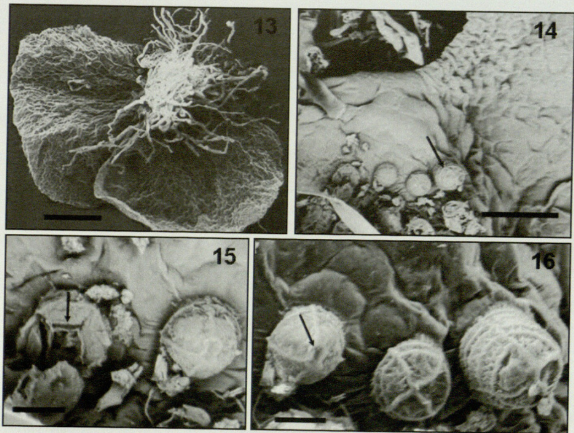
FIGS. 13–16. Scanning electron micrographs of Dicksonia sellowiana gametophytes. 13. General gametophyte view. Bar = 500 \mu m. 14. Aspects of inferior face bearing archegonia. Bar = 100 \mu m. 15. Detail of an archegonia. Bar = 20 \mu m.
