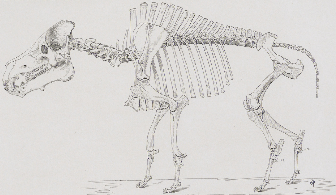
MOUNTED SKELETON OF Dinohyus hollandi PETERSON. \frac{1}{18} NAT. SIZE. ( ps , Palmar sesamoid.)
