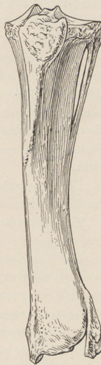
FIG. 77. Anterior View of Tibia-fibula of Type of D. hollandi Peterson. \frac{1}{4} nat. size.
