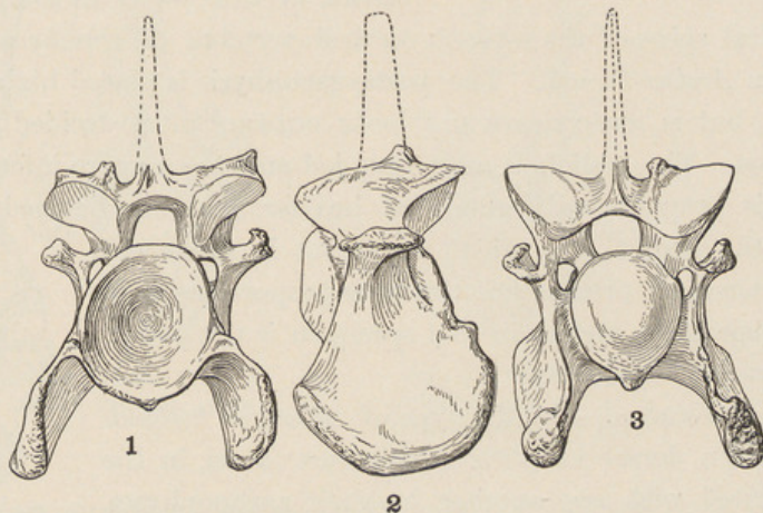
FIG. 42. Posterior (1), Lateral (2), and Anterior (3) Views of the Sixth Cervical of D. hollandi Peterson. \frac{1}{2} nat. size.
