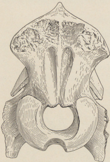
FIG. 3. Posterior View of Skull of Entelodon magnum Aymard. \frac{1}{2} nat. size. (Drawn by Sidney Prentice after the Figure given by Kowalevsky.)
