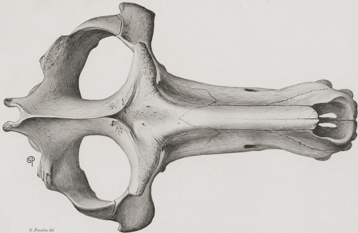
SUPERIOR VIEW OF CRANIUM OF Dinohyus hollandi PETERSON. \frac{7}{25} NAT. SIZE.
