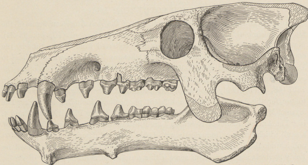
FIG. 4. Side View of Skull of Archæotherium mortoni Leidy. (Carn. Mus. Cat. Vert. Foss. Skull No. 1900, Lower Jaw No. 2097.) \frac{1}{3} nat. size.
