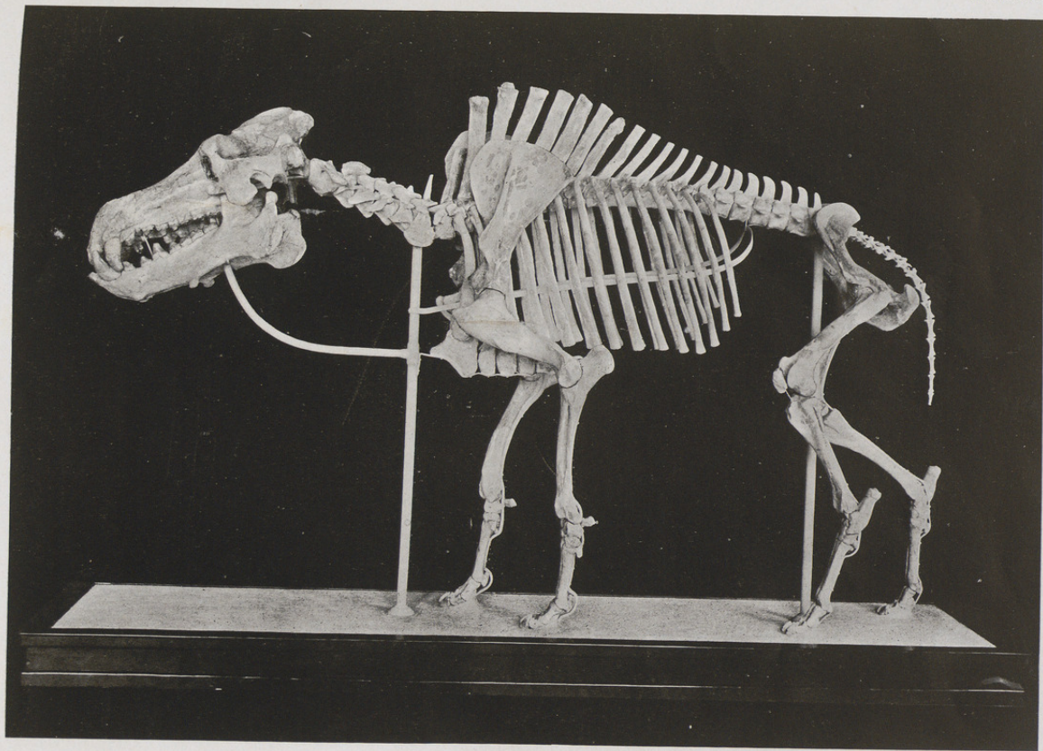
PHOTOGRAPHIC REPRODUCTION OF THE MOUNTED SKELETON OF Dinohyus hollandi PETERSON. ABOUT \frac{1}{15} NAT. SIZE.
