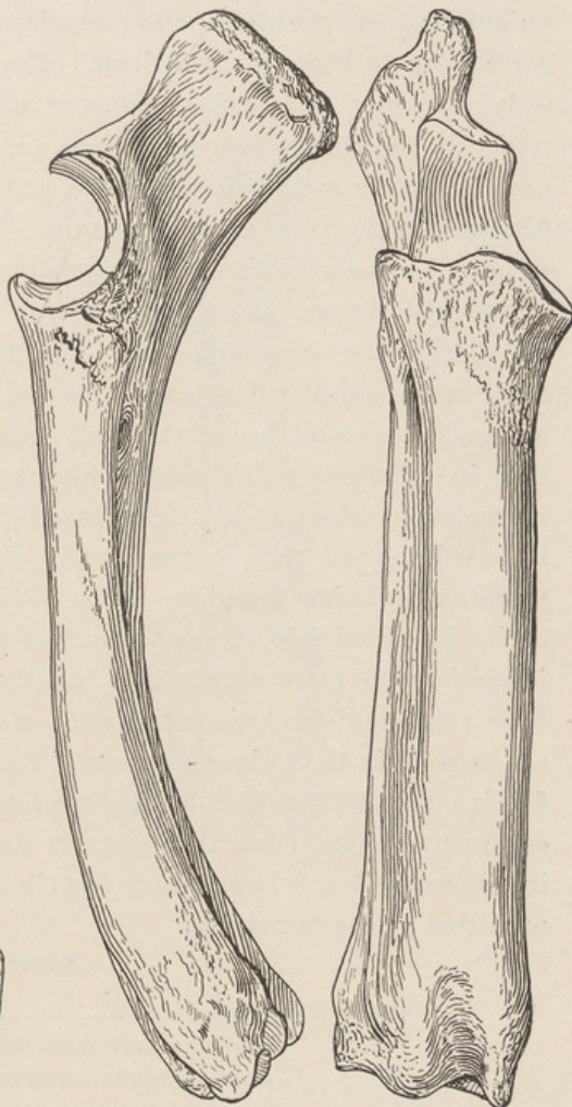
FIG. 69. Radial and Anterior Views of the Ulna-radius of Type of D. hollandi Peterson. \frac{1}{2} nat. size.
