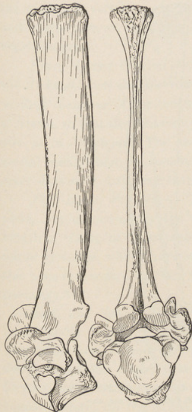
FIG. 45. Lateral and Posterior Views of First Dorsal of D. hollandi Peterson. \frac{1}{4} nat. size.
