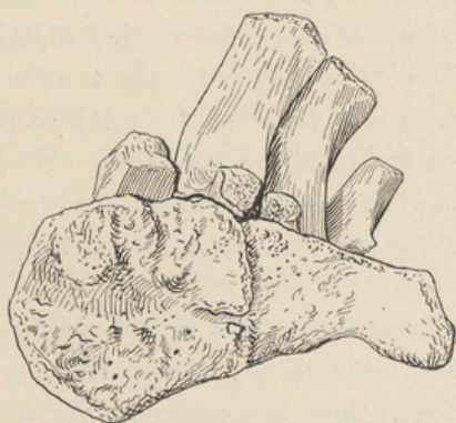
FIG. 62. Lateral View of Sacrum of D. hollandi Peterson. \frac{2}{3} nat. size. (Carn. Mus. Cat. Vert. Foss., No. 2126.)
