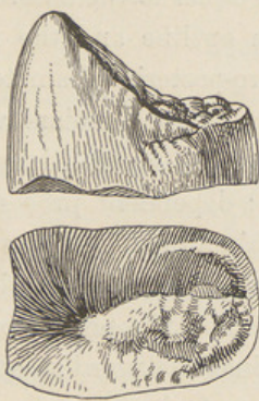
FIG. 20. Type of Ammodon leidy-anum Marsh. Internal and Crown View of P_4 . \frac{2}{3} nat. size. (Collection Yale Museum, No. 12040.)
