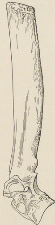
FIG. 49. Lateral View of Fifth Dorsal of D. hollandi Peterson. \frac{1}{2} nat. size.
