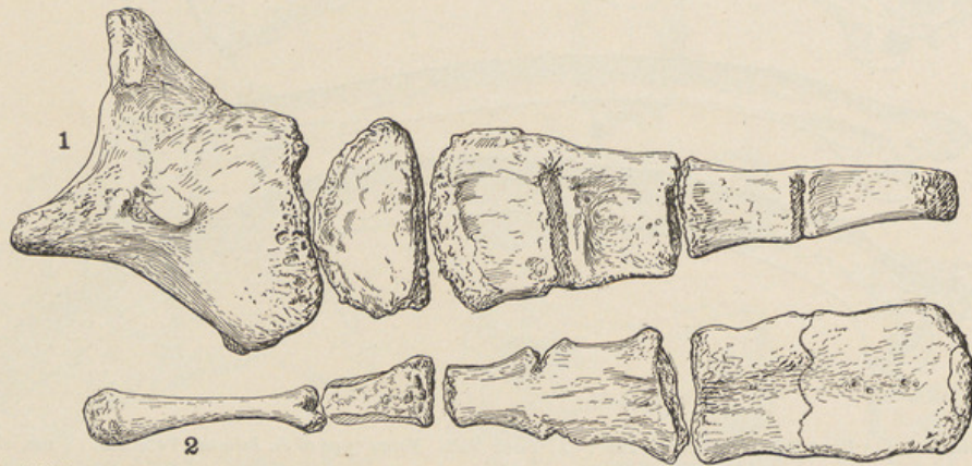
FIG. 66. (1) Lateral View of Sternum. (2) Inferior View of Sternum. Type of D. hollandi Petersén. \frac{1}{4} nat. size.
