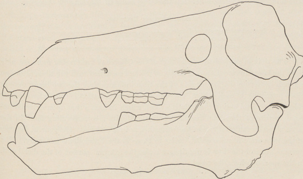
FIG. 19. Outline of Illustration of Skull of Deodon calkinsi (Sinclair). (After Sinclair.)
