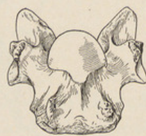
FIG. 44. Inferior View of Seventh Cervical of D. hollandi Peterson. \frac{1}{4} nat. size.
