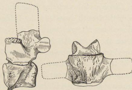
FIG. 57. Lateral and Inferior Views of Third Lumbar of D. hollandi Peterson. \frac{1}{3} nat. size.
