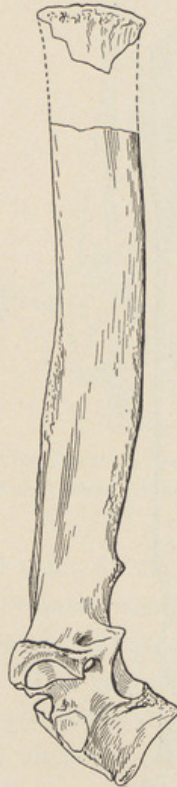
FIG. 48. Lateral View of Fourth Dorsal of D. hollandi Peterson. \frac{1}{2} nat. size.
