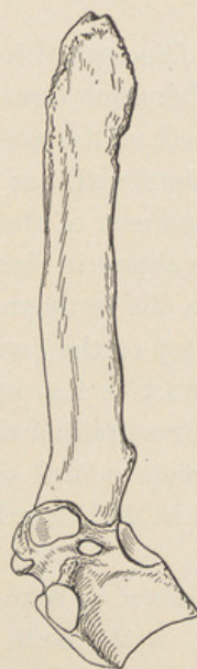
FIG. 51. Lateral View of Seventh Dorsal of D. hollandi Peterson. \frac{1}{4} nat. size.
