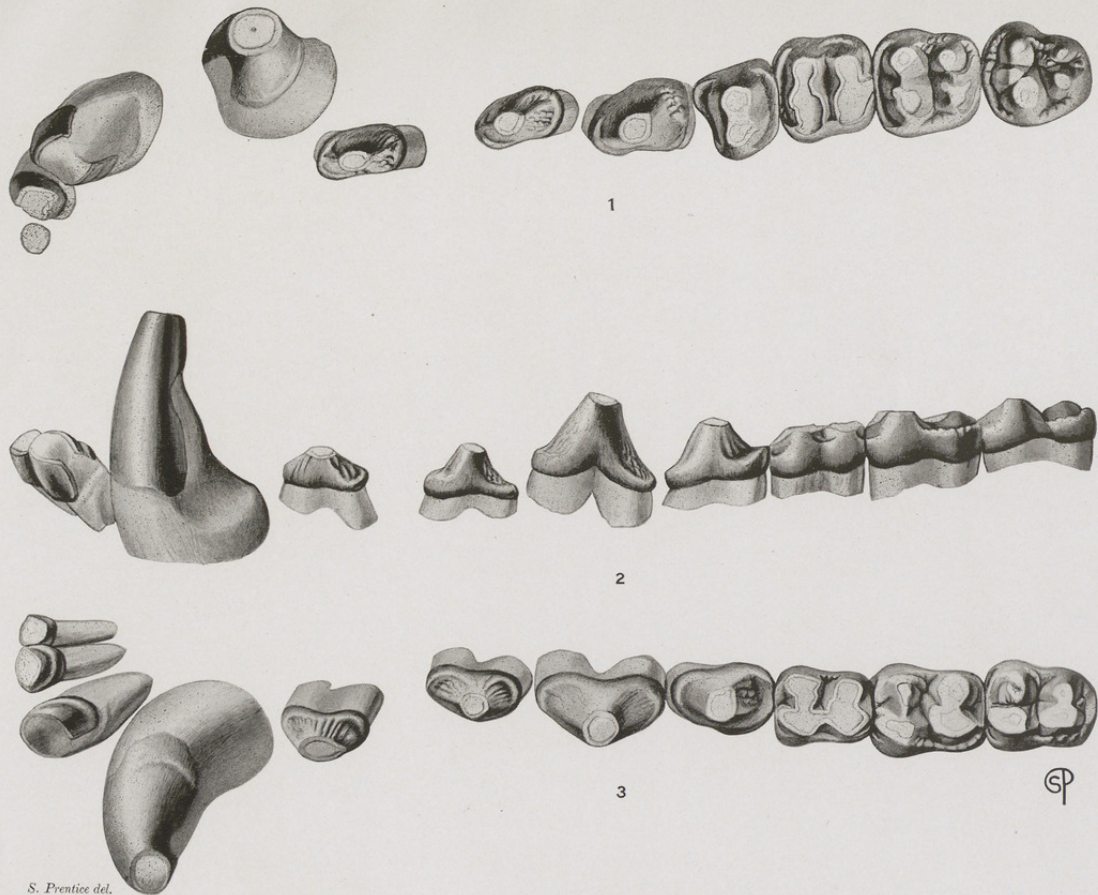
DENTITION OF Dinohyus hollandi PETERSON. \frac{1}{2} NAT. SIZE. 1. CROWN VIEW OF UPPER DENTITION OF LEFT SIDE. 2. SIDE VIEW OF LOWER DENTITION OF LEFT SIDE. 3. CROWN VIEW OF LOWER DENTITION OF LEFT SIDE.
