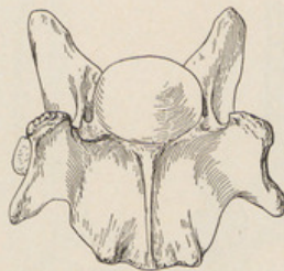
FIG. 41. Inferior View of Fifth Cervical of D. hollandi Peterson. \frac{1}{2} nat. size.
