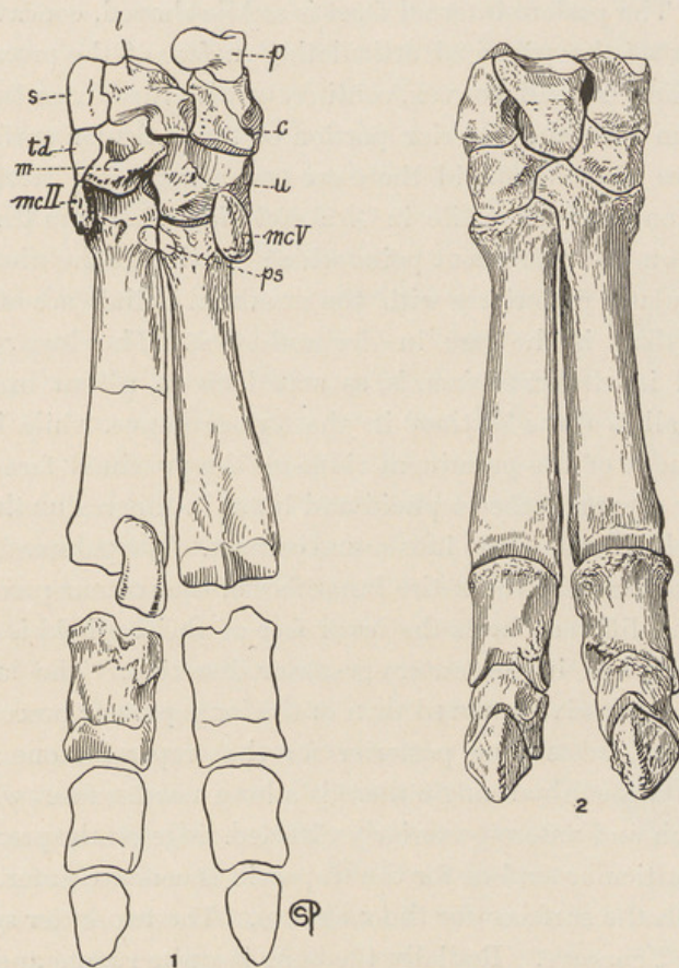
FIG. 70. Posterior (1) and Anterior (2) Views of the Right Fore Foot of Type of D. hollandi Peterson. \frac{1}{3} nat. size. ps, facets for palmar sesamoid.
