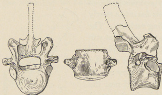
FIG. 54. Anterior, Inferior, and Lateral Views of Fourteenth Dorsal of D. hollandi Peterson. \frac{1}{3} nat. size.
