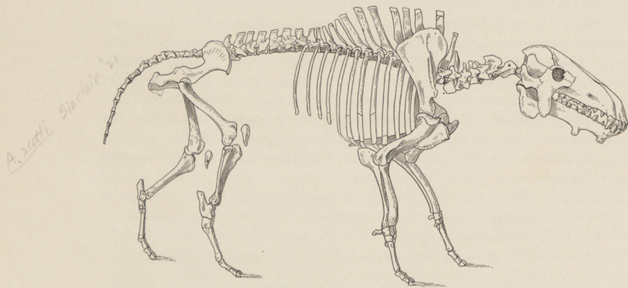
FIG. 9. Restoration of Skeleton of A. ingens Leidy. About \frac{1}{18} nat. size. (After Scott.)
