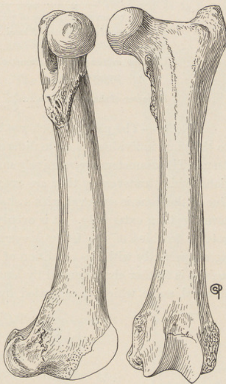
FIG. 75. Internal and Anterior Views of Femur of Type of D. hollandi Peterson. \frac{1}{2} nat. size.
