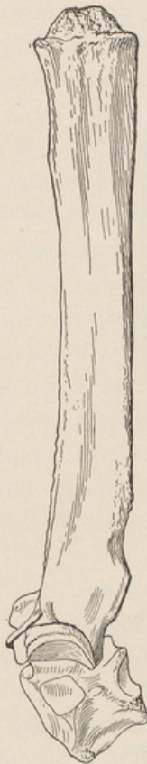
FIG. 46. Lateral View of Second Dorsal of D. hollandi Peterson. \frac{1}{4} nat. size.
