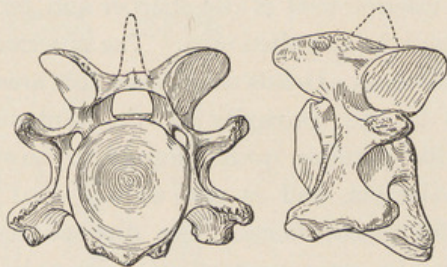
FIG. 40. Posterior and Lateral Views of Fifth Cervical of D. hollandi Peterson. \frac{1}{2} nat. size.
