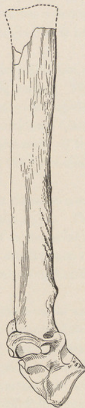
FIG. 47. Lateral View of Third Dorsal of D. hollandi Peterson. \frac{1}{4} nat. size.
