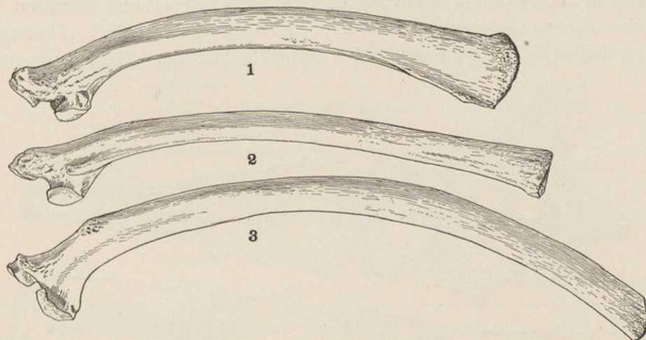
FIG. 65. (1) First Rib; (2) Second Rib; (3) Fifth Rib. From type of D. hollandi Peterson. \frac{1}{4} nat. size.
