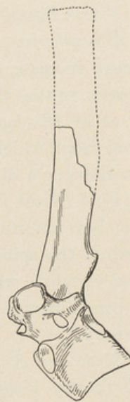
FIG. 52. Lateral View of Eighth Dorsal of D. hollandi Peterson. \frac{1}{4} nat. size.
