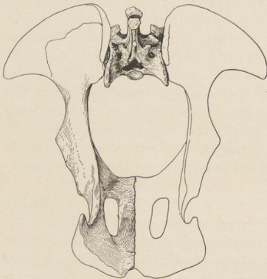
FIG. 73. Superior View of Pelvis of D. hollandi Peterson. \frac{1}{2} nat. size. (Carn. Mus. Cat. Vert. Foss., No. 2126.)
