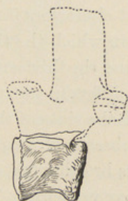
FIG. 56. Lateral View of Second Lumbar of D. hollandi Peterson. \frac{1}{3} nat. size.
