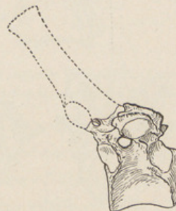
FIG. 53. Lateral View of Thirteenth Dorsal of D. hollandi Peterson. \frac{1}{4} nat. size.
