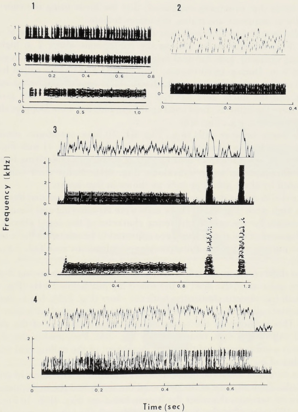
FIG. 3. Analyses of Bonin Petrel calls using an extended time scale. (1) Top: a churr analysed at half speed and (bottom) tape played at normal speed. Middle spectrograph used a narrow band filter, upper one a wide band filter; both show that call was composed of a series of rather regular pulses. (2) Part of an analysis of the churr of Fig. 2(4) slowed down four times. The amplitude trace (top) and the wide band analysis (bottom) emphasize the pulsed character of this call. (3) Bottom: a slowed down churr followed by two ti-ti calls from the same bird. The churr seems to be based on a series of very close harmonics (narrow band analysis) but the broad band and amplitude traces above show that the call is made from very fine pulses. (4) The low aerial moan of Fig. 4(3) is also composed of a rapid succession of pulsed sounds.
