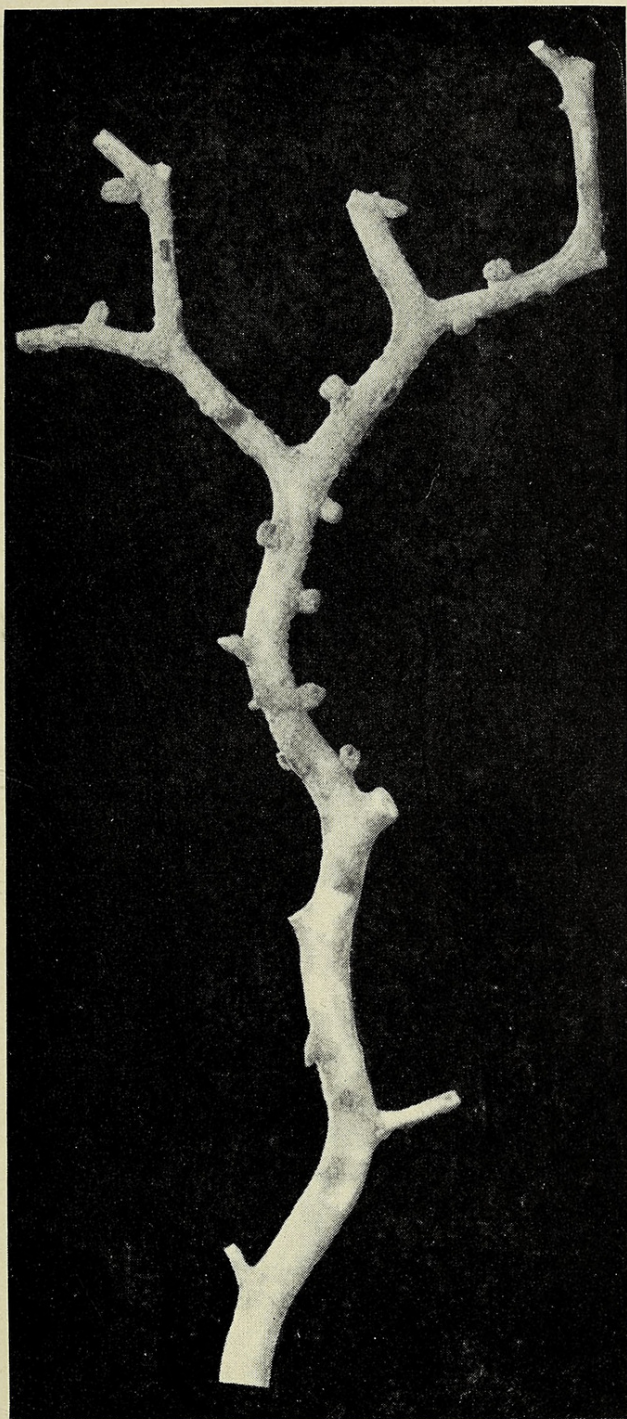
FIG. 4. Corallium abyssale sp. nov. The type specimen.
