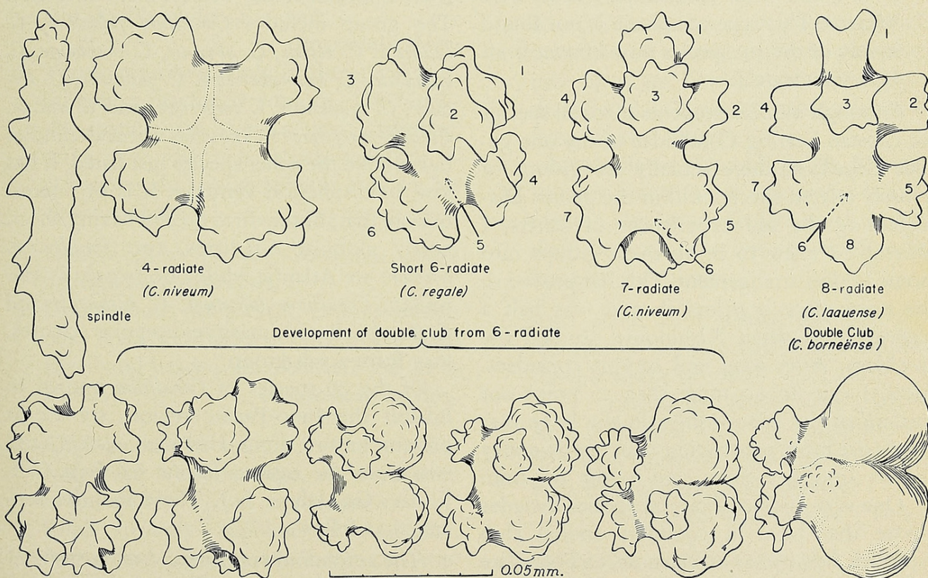
FIG. 3. Spicule types in the genus Corallium .
