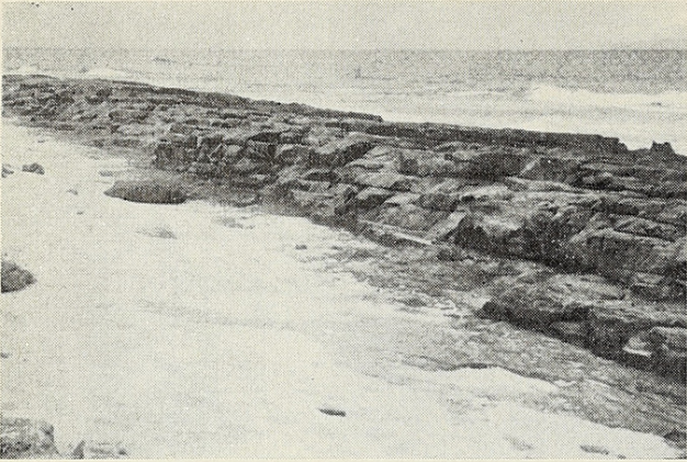
FIG. 11. Bar-like ridge of seaward-dipping beachrock just beyond beach of loose sand at Nohili, Kauai.
