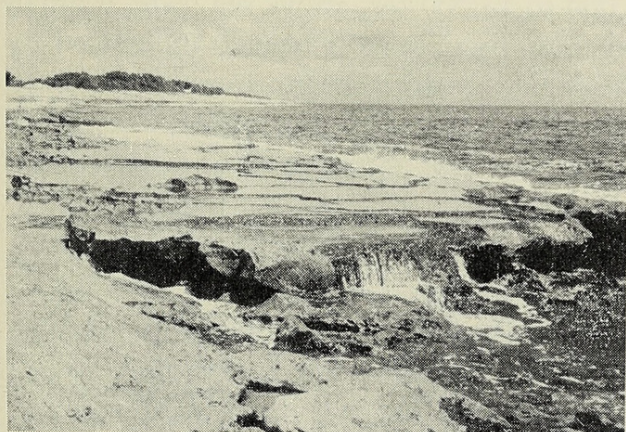
FIG. 9. Rimmed terraces in beachrock at Nohili, Kauai. Note narrow anastomosing ridges that separate the pools of different levels. These consist of beachrock, showing that the rimmed terraces are erosional rather than built up by deposition. Beachrock extends several feet, at least, below low water.
