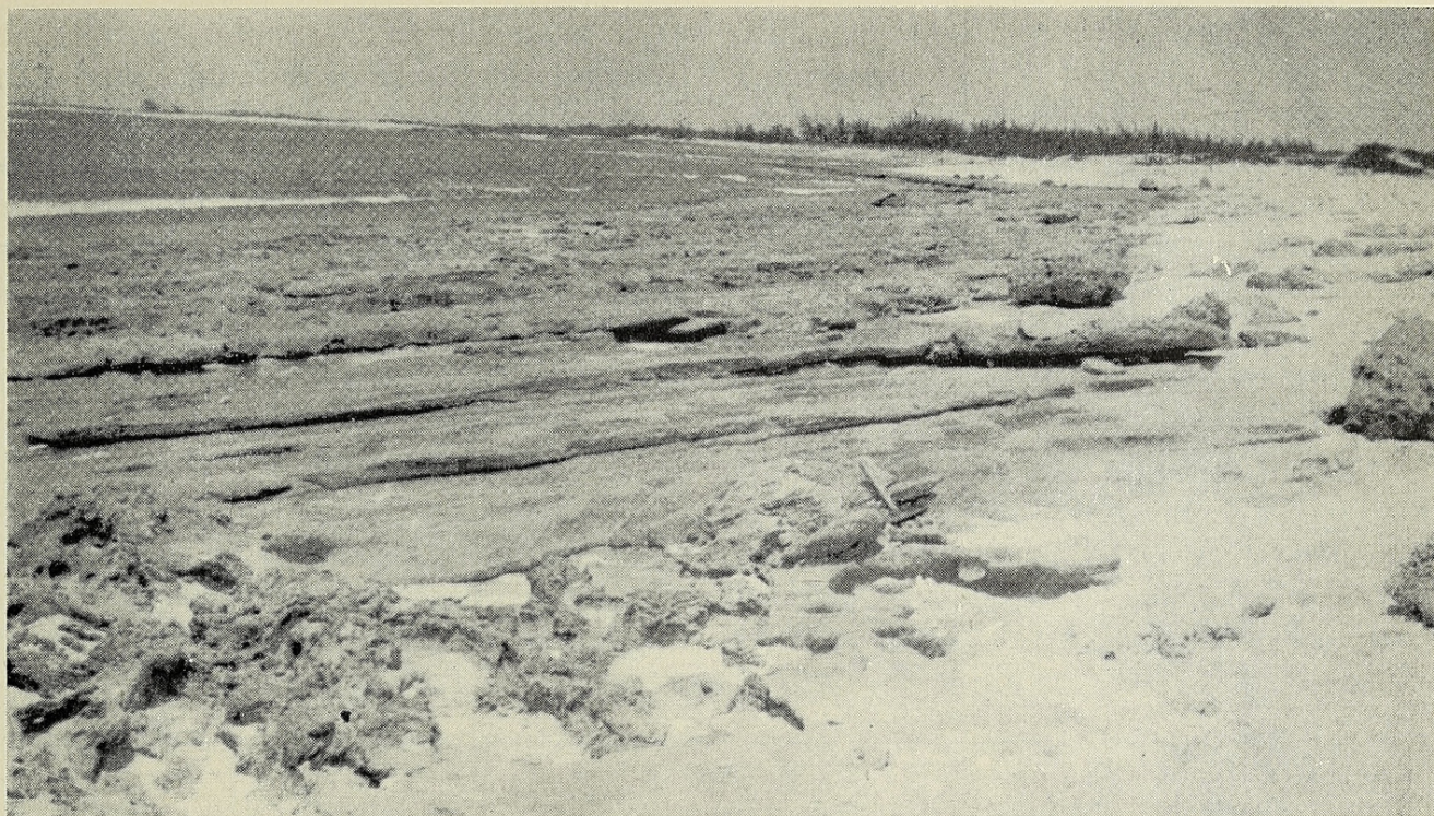
FIG. 4. Layered beachrock dipping seaward at west side of small bay west of Kahuku Point, Oahu. Note reef rock on left against which beachrock abuts. Site of measurements diagrammed in Figure 5 is at left center.
