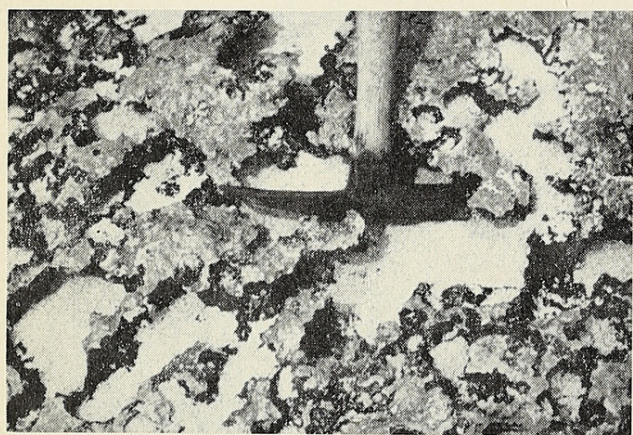
FIG. 7. Solution basins in beachrock having a case-hardened surface formed by deposition of a thin film of calcium carbonate at a place \frac{1}{2} mile north of Nanakuli, Oahu.
