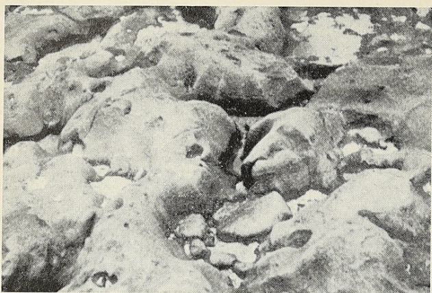
FIG. 15. Beachrock at Nohili, Kauai, showing solution basins having rounded and smoothed surfaces believed to indicate modification of ordinary sharp-edged solution basins during a period of burial under loose beach sand followed by exhumation.
