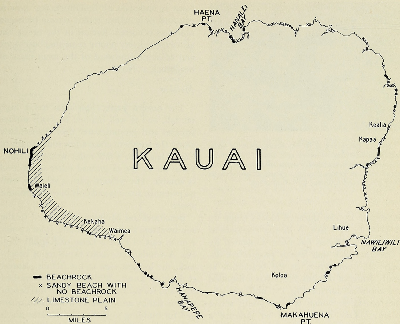
FIG. 14. Distribution of beachrock on Kauai.
