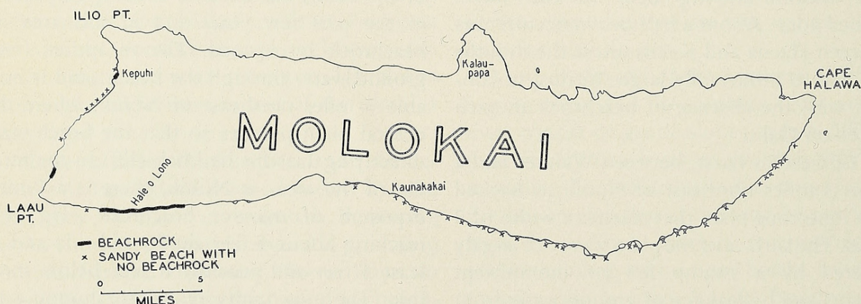
FIG. 16. Distribution of beachrock on Molokai.
