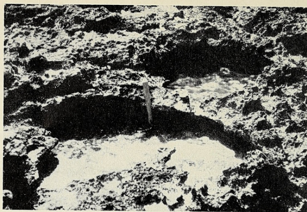
FIG. 8. Solution basins in reef rock \frac{1}{2} mile north of Mauna Lahilahi, Oahu. The reef rock surface is seen to be typically rougher than that of beachrock.
