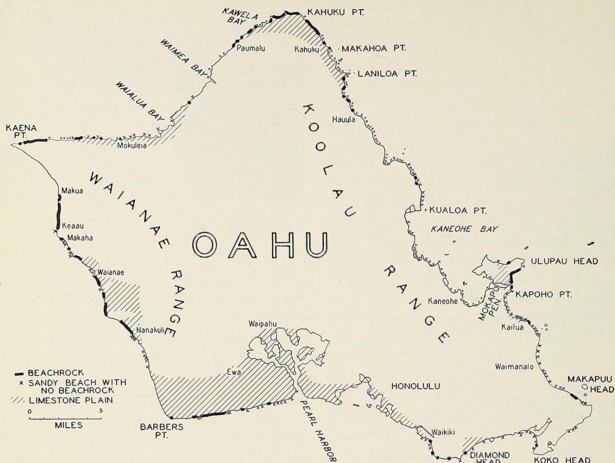
FIG. 12. Distribution of beachrock on Oahu.
