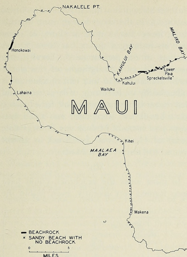
FIG. 17. Distribution of beachrock on Maui.
