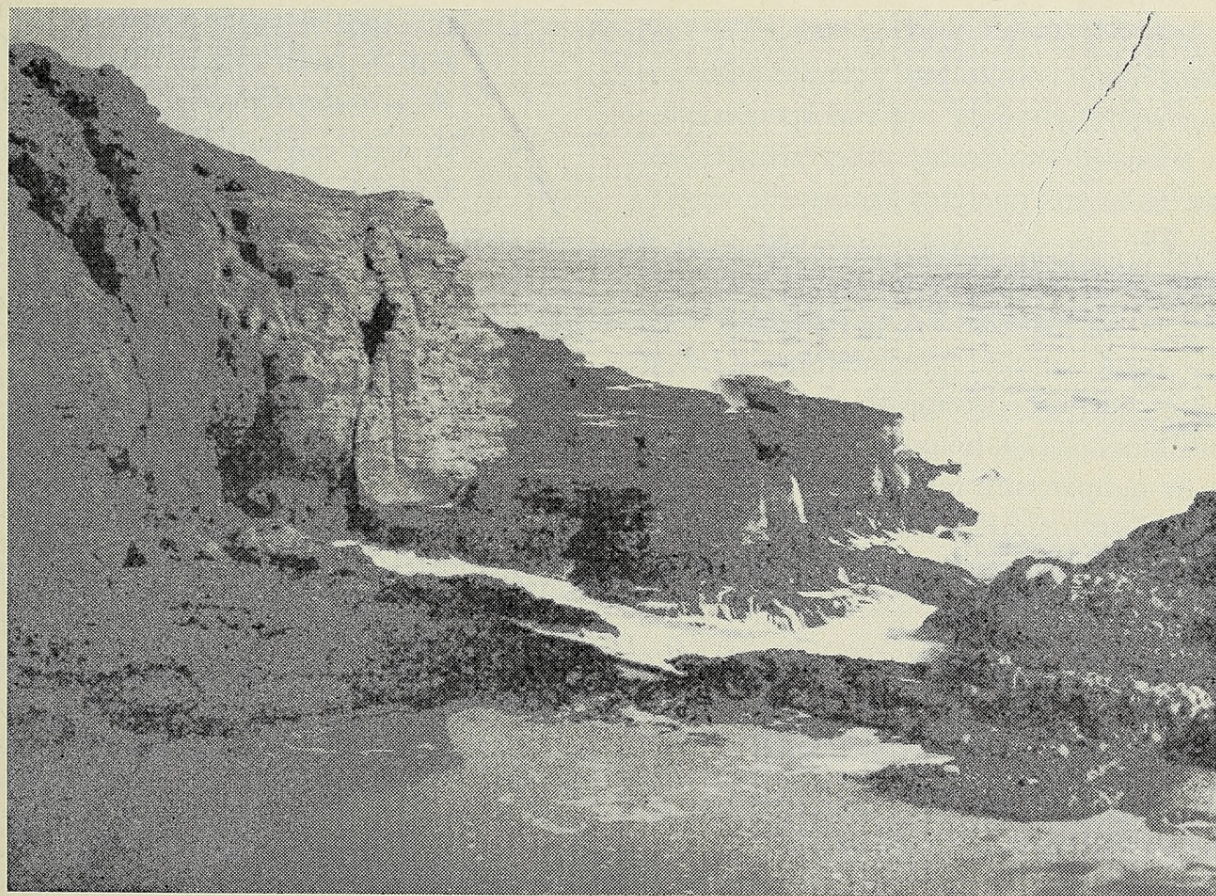
FIG. 2. Mouth of the gap, south of Camel Rock. Note the sharp upper limit to the algal zonation, most of which is Durvillea .
