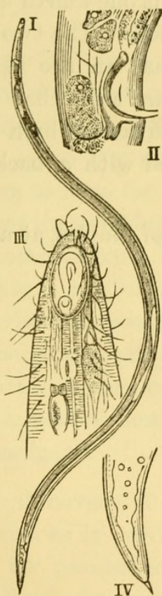
FIG. 9.—I, THE MALE OF DIPELTIS TYPICUS ( \times 40 ); II, III, and IV, the anal region, head and tail end, respectively, of the same worm, more highly magnified (II, \times 350 ; III, \times 450 ; IV, \times 350 ). I, shows, in the upper part, the oesophagus surrounded by the nerve-ring (white) and the unicellular excretory organ and its duct (both black); near the middle of the body the two (?) testicles (light).
