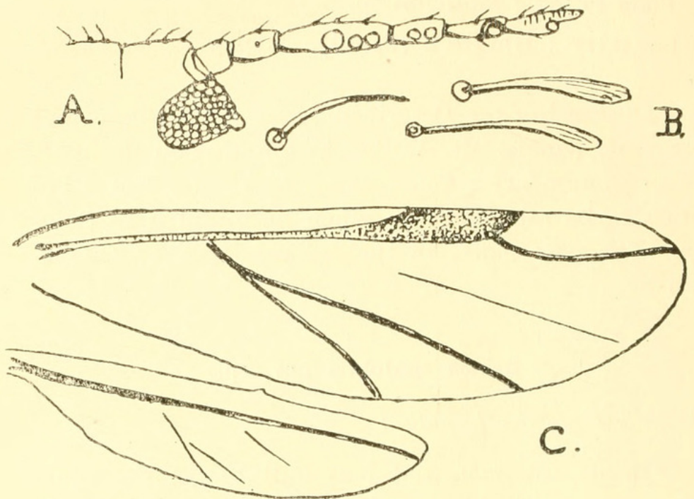
Geioica spatulata nov. sp., alate viviparous ♀. — A. Head, antenna and eye; B. Squamae; C. Wings.
