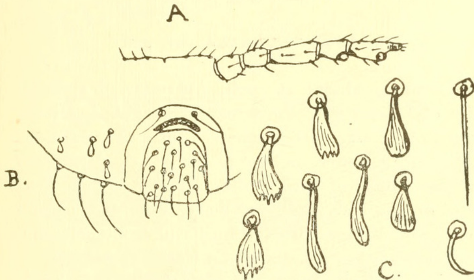
Geioica spatulata nov. sp., apterous viviparous ♀. — A. Head and antenna; B. Cauda and anal process; C. Squamae of body.
