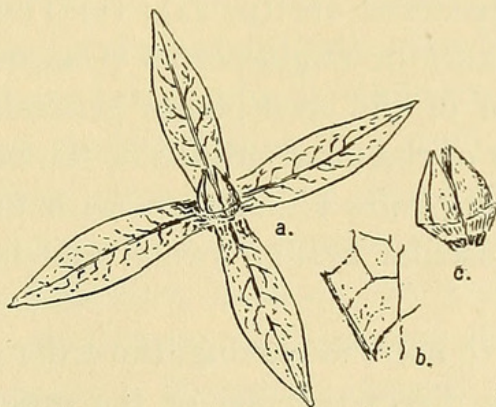
FIG. 1. Carpolithes macrophyllus . a, Whole fossil, the edges of the calyx-lobes restored; b, detail of venation; c, fruit.
