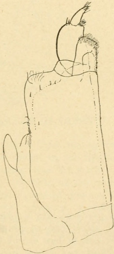
Text-fig. 10. Maxilliped.
