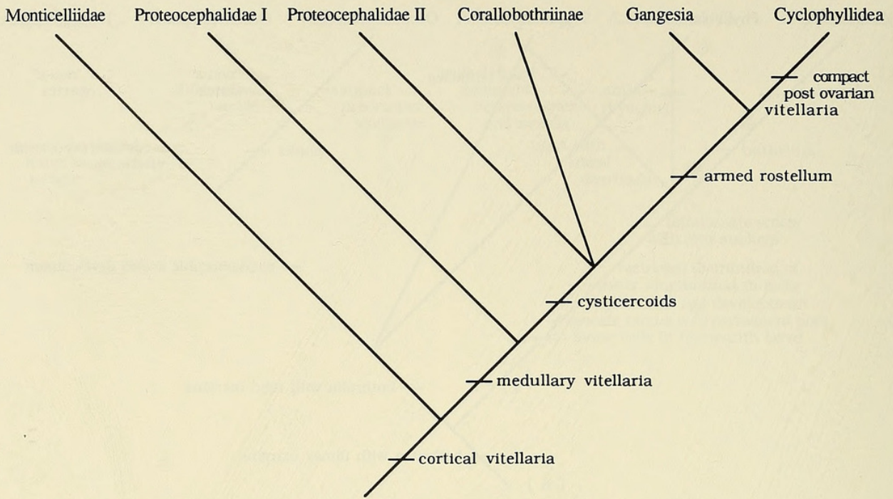
Fig. 3. Phylogenetic tree depicting relationships among members of the major groups of the proteocephalidean plus cyclophyllidean lineage based on the synapomorphic traits listed next to each slash mark on the tree.
