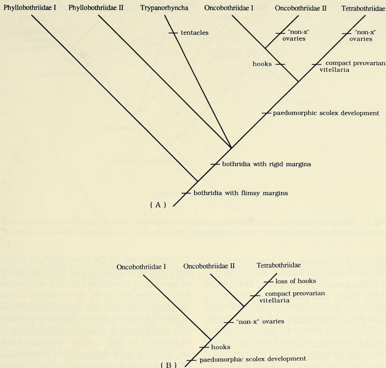
Fig. 2. (A) Phylogenetic tree depicting possible relationships among major groups of tetraphyllidean eucestodes based on the synapomorphic traits listed next to each slash mark on the tree. (B) Equally parsimonious alternative arrangement for the onchobothriids and tetrabothriideans.
