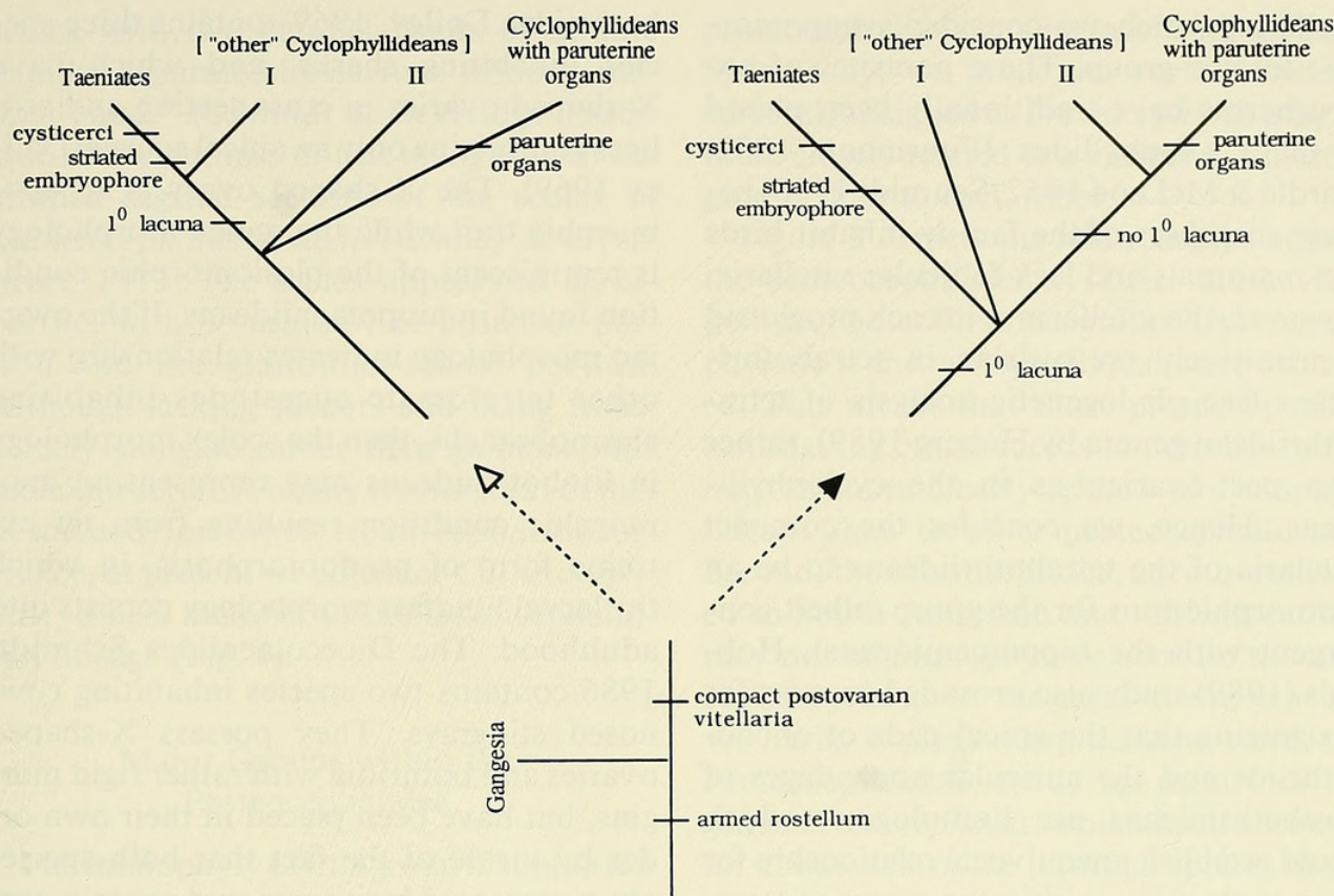
Fig. 4. Alternative phylogenetic trees depicting possible relationships of basal cyclophyllidean groups based on synapomorphic traits listed next to each slash mark on the tree.
