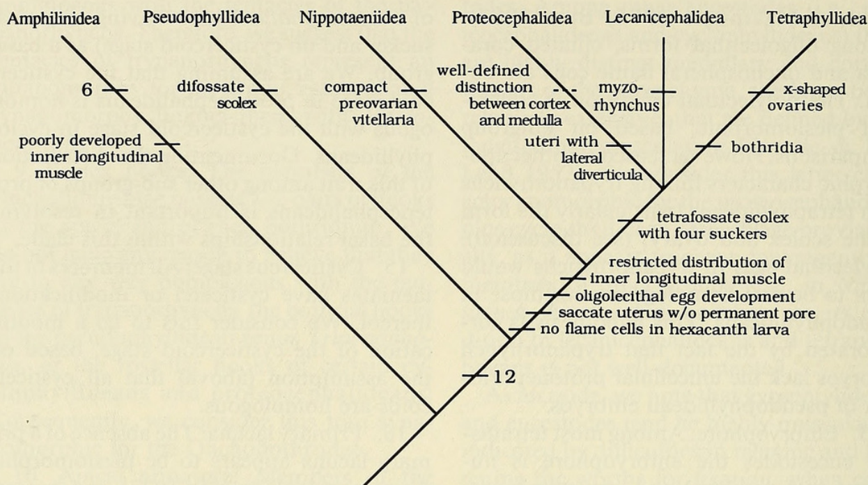
Fig. 1. Phylogenetic tree depicting five major groups of eucestodes based on the synapomorphic traits listed next to each slash mark on the tree. Numbers next to slash marks on the Amphilinidea line (sister-group) and the line uniting all eucestodes indicate number of synapomorphic traits supporting the monophyly of the groups.
