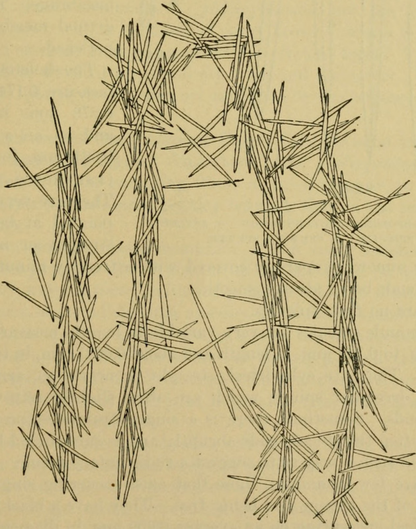
FIG. 2.—SPONGILLA PHILIPPINENSIS, FRAGMENT OF SKELETON, \times 70 .
