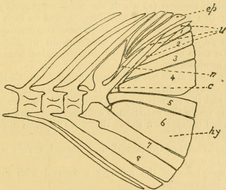
Skeleton of caudal fin of Chatoessus erebi .
