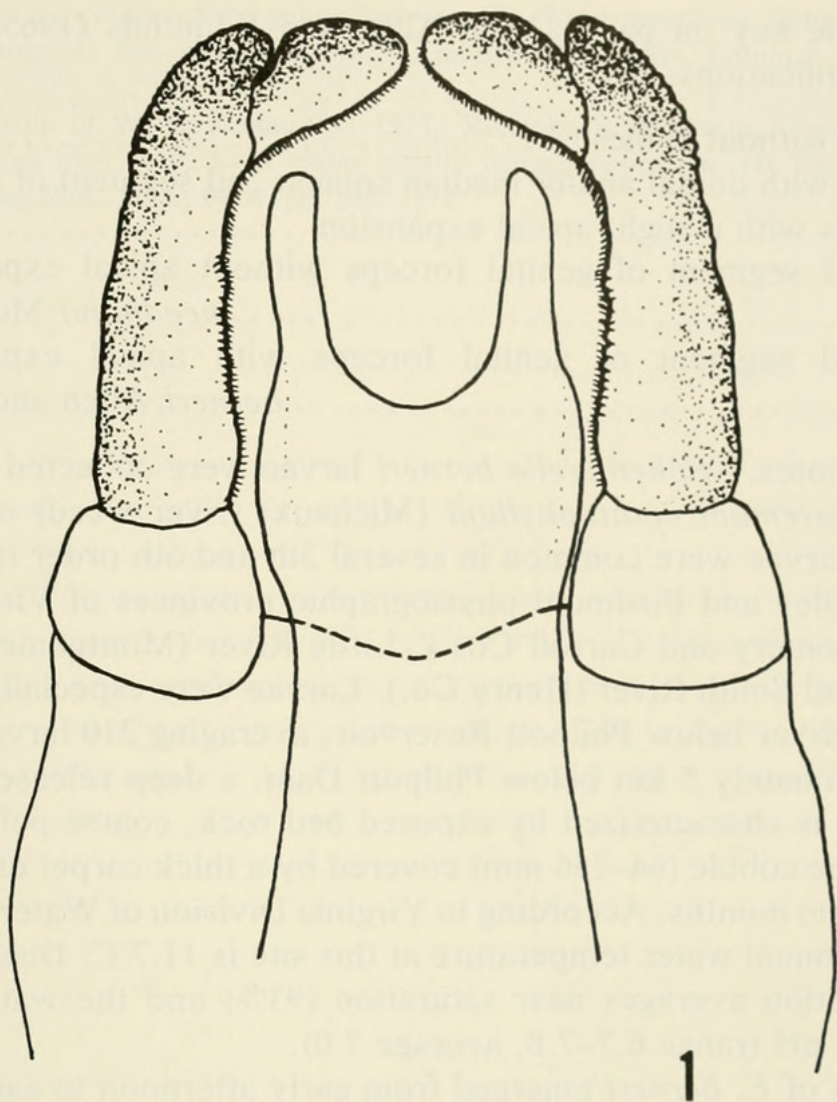
Fig. 1. Ephemerella bernerī , dorsal view of male genitalia.
