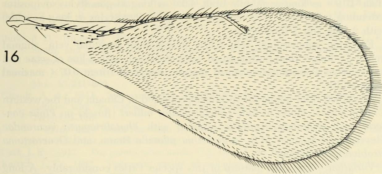
Fig. 16. Forewing of Zagrammosoma nigrolineatum .
