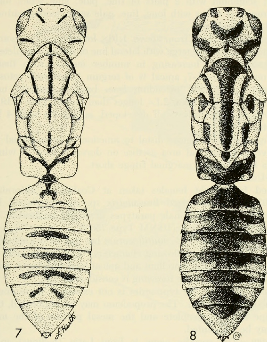
Figs. 7-8. Dorsal view of Zagrammosoma nigrolineatum .
