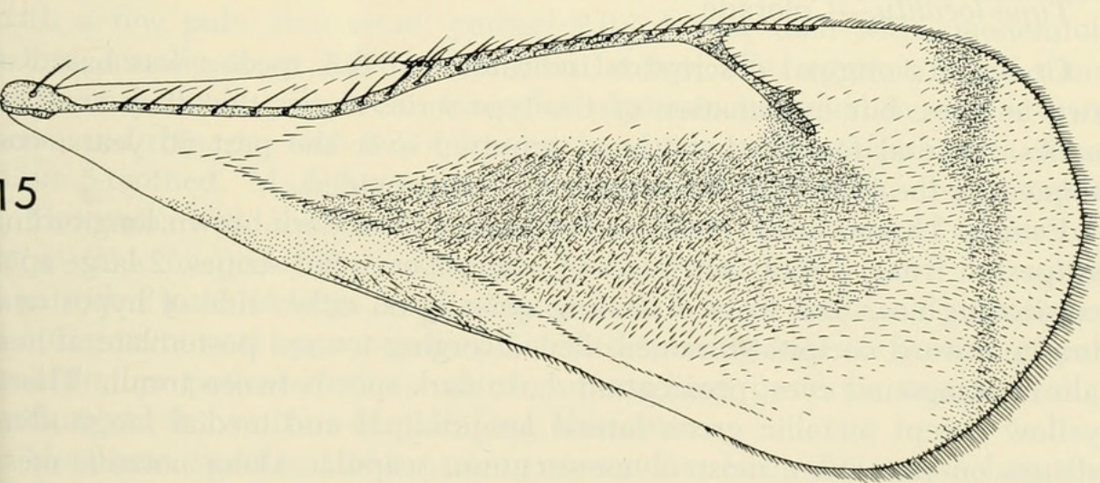
Figs. 13-15. Forewings of Zagrammosoma species. 13. Z. americanum ; 14. Z. melinum ; 15. Z. centrolineatum .
