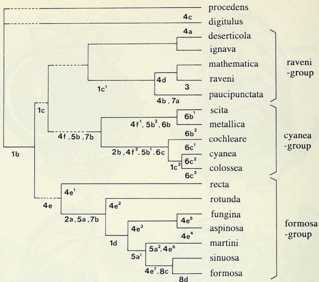
Fig. 4. Cladogram of the males of Storena .
