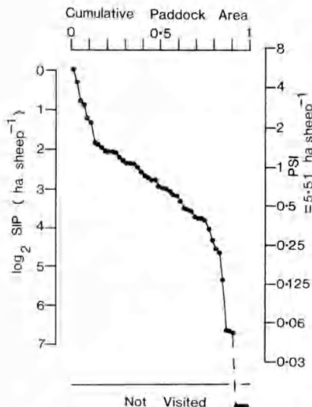
Fig. 3. The cumulative distribution of \log_2 SIP for the 50 parts of Overland Paddock June 1978-January 1979 inclusive (Study 4).
