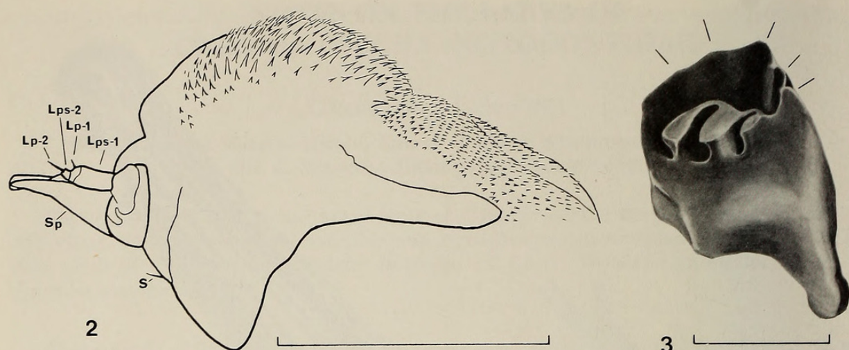
FIGS. 2 & 3. Cargida pyrrha : 2, hypopharyngeal complex, left lateral view (Lp-1 = seta on first segment of labial palpus, Lp-2 = seta on second segment of labial palpus, Lps-1 = first segment of labial palpus, Lps-2 = second segment of labial palpus, S = stipular seta, Sp = spinneret); 3, left mandible, oral view (leader lines mark positions of the five outer teeth). Scale lines = 0.5 mm. Descriptive terminology follows Godfrey (1972).
