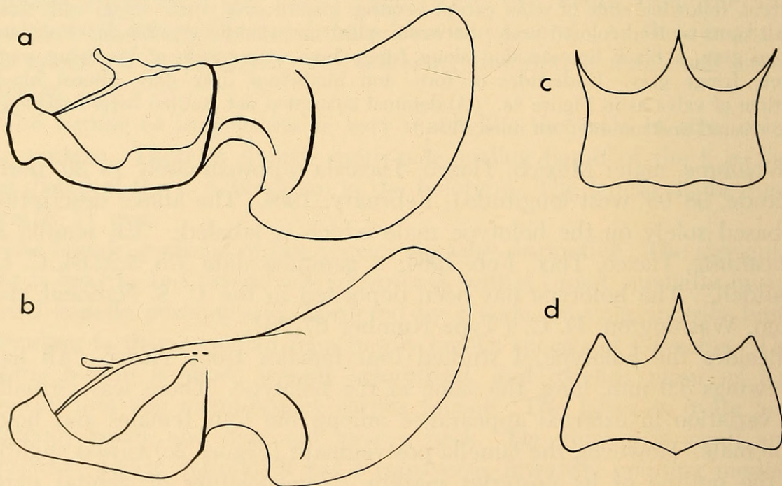
Fig. 2. Outline of genital parts of Laspeyresia species; (a) valva of L. nigra Miller, holotype; (b) valva of L. miscitata Heinrich, holotype; (c) lamella postvaginalis of L. nigra ; (d) lamella postvaginalis of L. miscitata .
