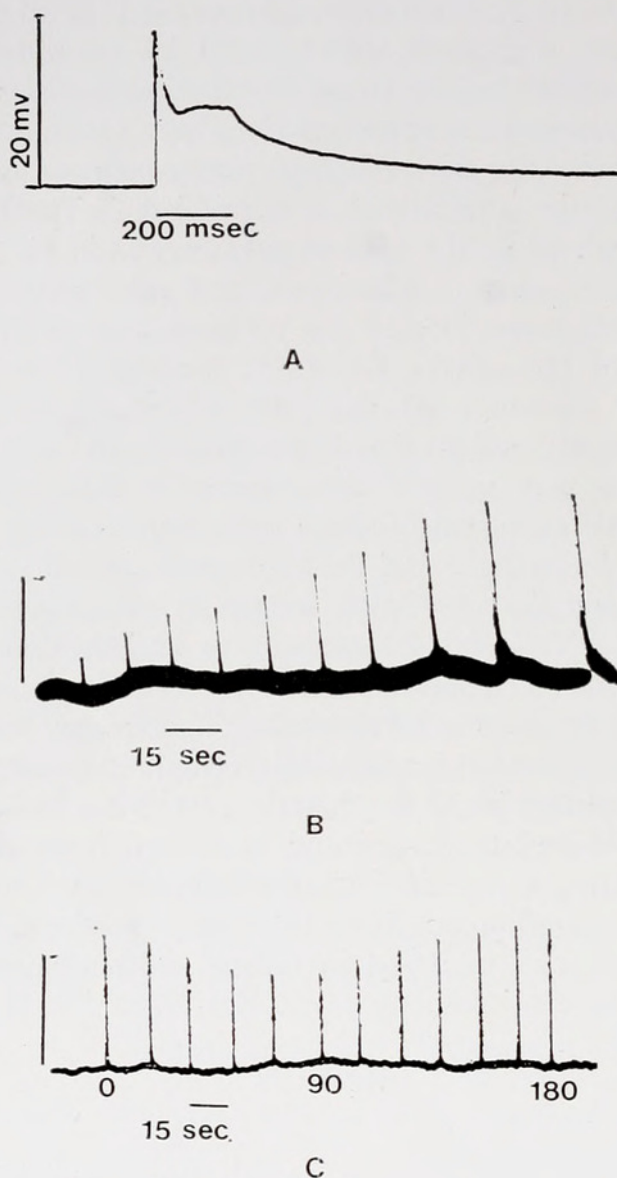
FIGURE 1. Response of a single reticular cell to (a) a 200 msec flash of light of moderate intensity; (b) response of the same cell to a series of 40 msec light flashes of increasing intensity. Each flash is twice (0.3 log units) as bright as the preceding flash and the interval between flashes is 15 seconds; (c) the response of the cell to a series of polarized stimuli of constant intensity and 40 msec duration delivered at an interval of 15 sec. During the interval the polarizing filter was rotated 15^\circ . (The vertical calibration is the same for A, B and C.) The numerals below the trace indicate the cells' response to polarization angles of 90 and 180 degrees.
