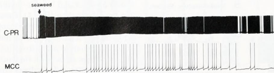
Figure 6. Example of a prolonged excitatory response in C-PR and the MCC to a brief seaweed stimulus. Calibration: 5 s, 20 mV. Data from Teyke et al. (1990a).
