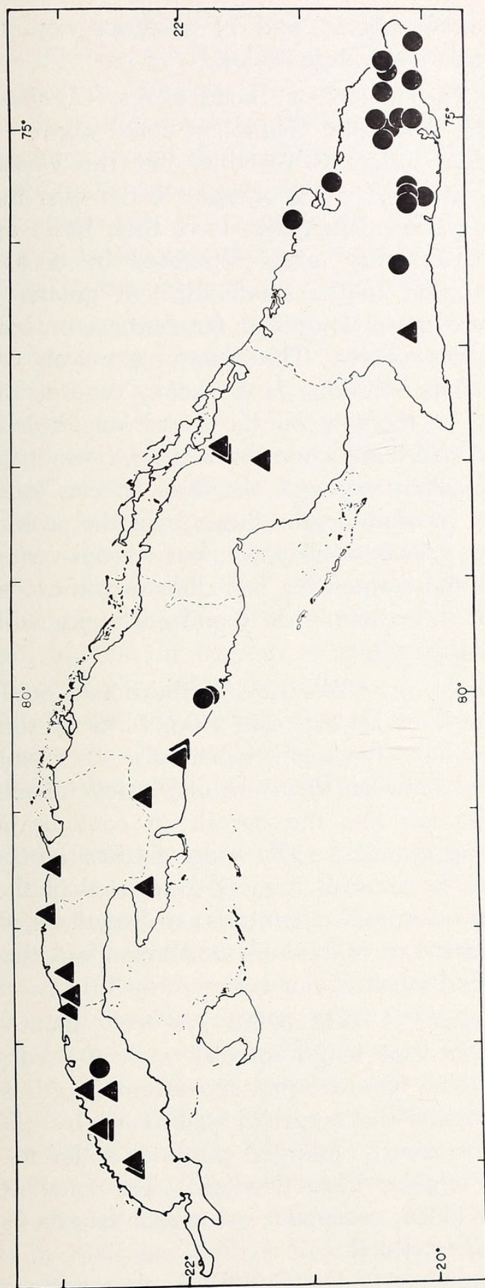
Fig. 2. Map of Cuba, showing distribution of two species of Chamaeleolis . Triangles, C. chamaeleonides ; circles, C. porcus .
