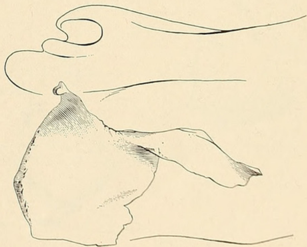
FIG. 1.— Dinichthys cf. terrelli Newberry (U.T.-B.E.G. no. 40100): Left paranuchal plate fragment in internal aspect. Reproduction approx. \times 2/5 .
