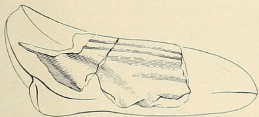
FIG. 4— Dinichthys cf. terrelli Newberry (U.T.-B.E.G. no. 40100-1): Right interolateral plate fragment in anterolateral aspect. Reproduction approx. \times 2/5 .
