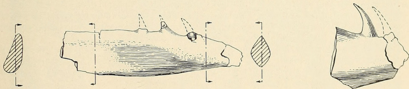
FIG. 5.— Arthrodira , gen. and sp. undet. (U.T.B.E.G. no. 40101): Fragments of dentate mandibular elements in transverse sections and lateral aspects. Reproduction approx. \times 9/10 .
