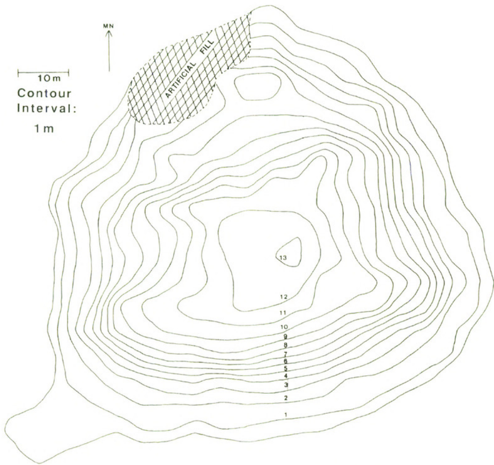
Figure 1. Bathymetric map of Arcadia Bog.
