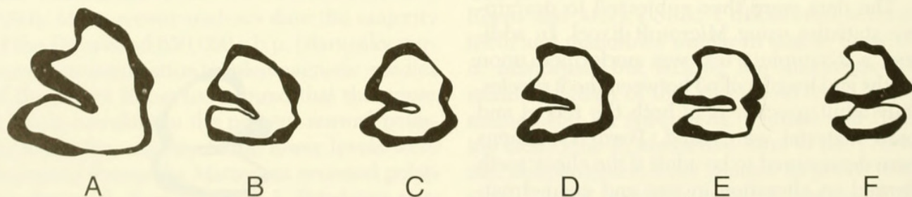
Fig. 3. Comparison of p3 enamel patterns for Hypolagus , B. coloradoensis , and B. idahoensis . A is Hypolagus (redrawn from White 1987:439), B–E (DMNH # unknown, DMNH #33257, DMNH #33255, and DMNH #33260) represent the range of variation seen in specimens of B. coloradoensis . B predominates slightly in earlier sediments whereas C becomes somewhat more plentiful in younger sediments at Porcupine Cave. F is that of B. idahoensis (UCM #5840). Note also that some specimens of B. coloradoensis have a slight posterior-internal reentrant (PIR).
