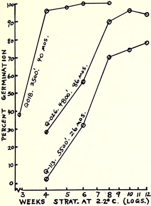
FIG. 4. Length of stratification and germination of deerbrush ( Ceanothus integerrimus ) seeds. (Seed collection number, altitude of collection, and seed age in months.)
