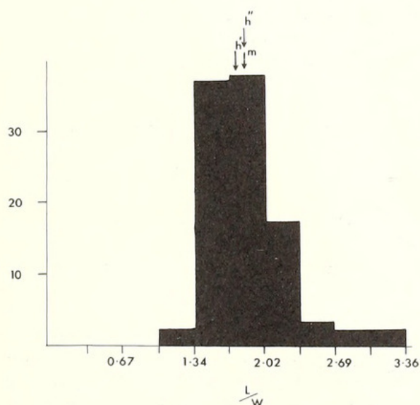
TEXT-FIG. 4. Histogram showing the frequency of the L/W parameter in the topotype material h' , h'' , and m as in text-fig. 3. F calculated as percentages of the total. Standard deviation of L/W is 0.36.
