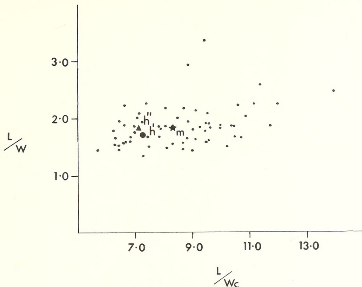
TEXT-FIG. 3. Scatter diagram of the topotype material based upon sixty-five complete specimens. h' —holotype of Rhaetogonyaulax rhaetica ; h'' —holotype of R. chaloneri ; m —mean. The diagram has a correlation coefficient of 0.3706.
