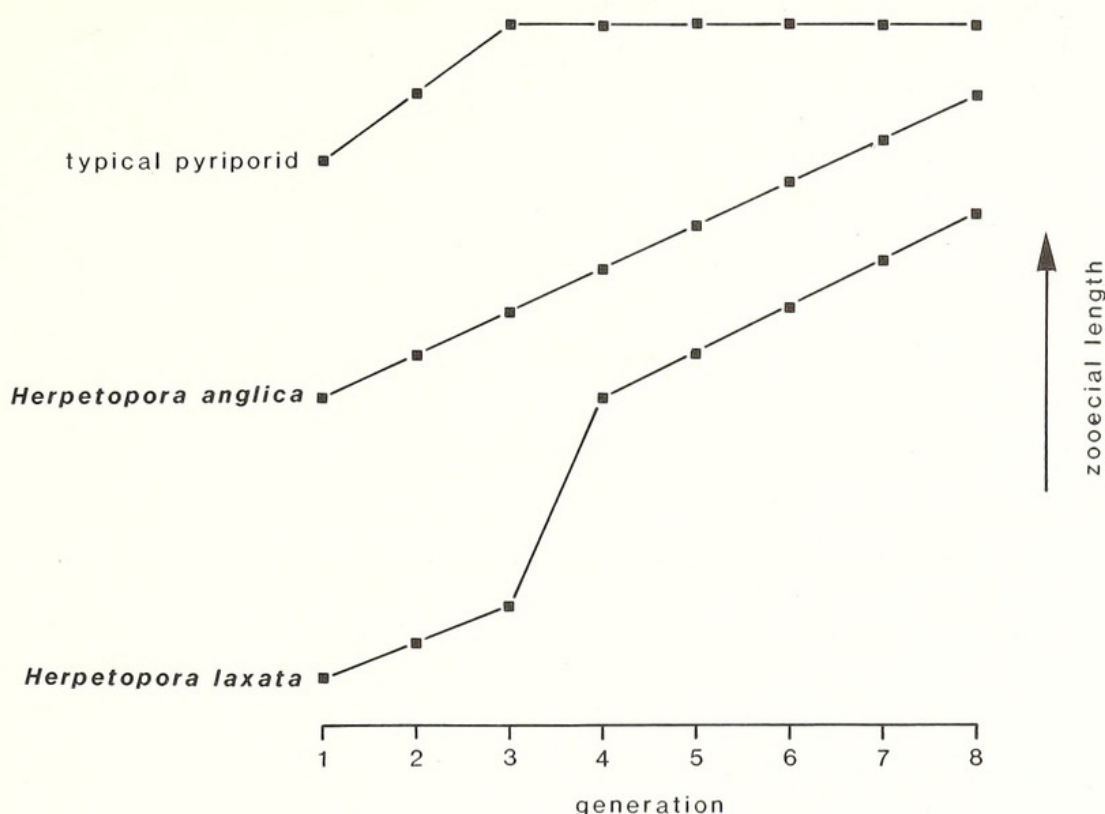
TEXT-FIG. 13. Simplified astogenetic gradients present in branches of typical pyriporid cheilostomes, Herpetopora anglica , and H. laxata .
