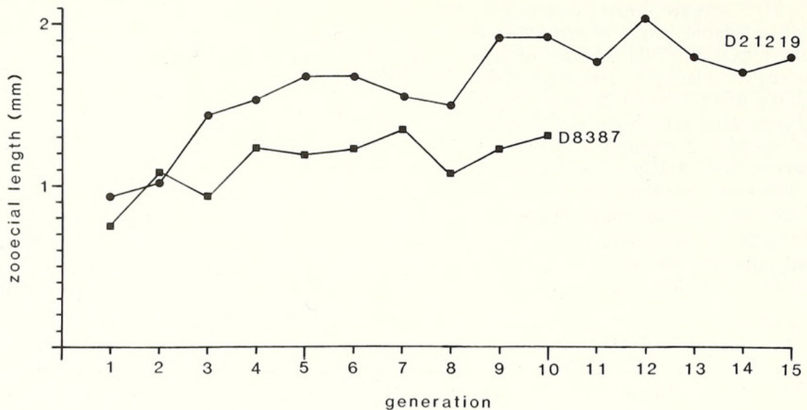
TEXT-FIG. 12. Astogenetic gradients of autozooidal length in long branches from two BM(NH) colonies of Herpetopora anglica .
