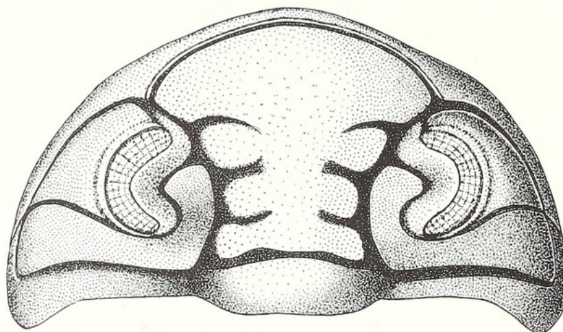
TEXT-FIG. 2. Pterygometopus sclerops (Dalman, 1827). Reconstruction of cephalon in dorsal view showing course of facial suture; based on lectotype RM Ar18074 (Pl. 1, fig. 2); lower Hølen Limestone, Kunda Stage, probably lower Asaphus raniceps Zone; Husbyfjöl (Västana), Östergötland, Sweden; \times 4 .
