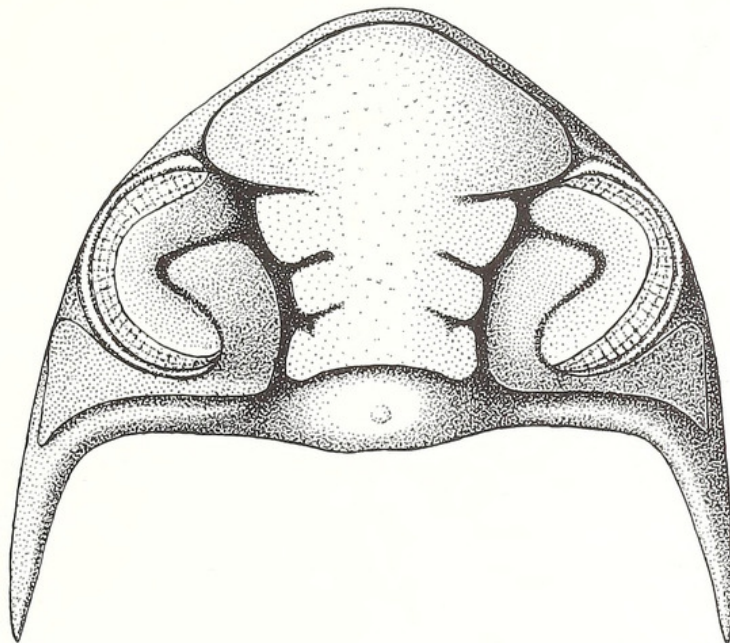
TEXT-FIG. 3. Ingriops trigonocephalus (Schmidt, 1881). Reconstruction of cephalon in dorsal view, based on syntype RM Ar38514 (Pl. 5, fig. 1); Voka Beds?, Kunda Stage ( Didymograptus artus Zone); Pavlovsk, Ingria, western Russia; \times 4 .
