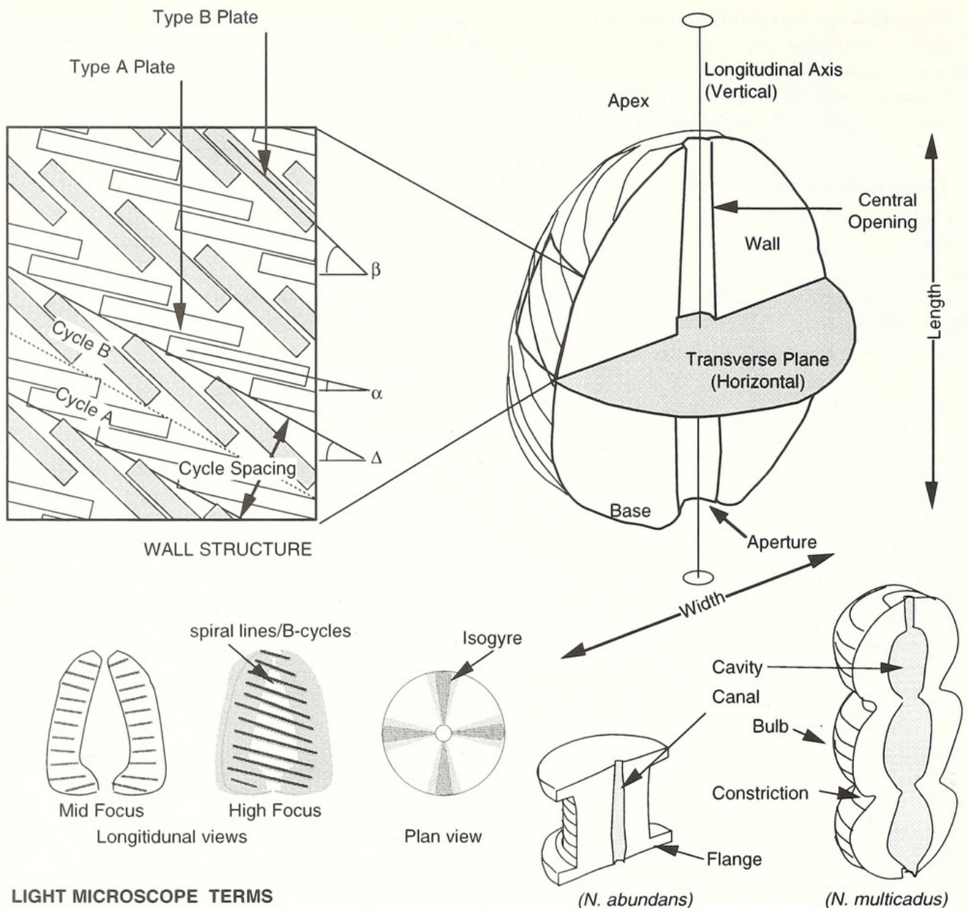
TEXT-FIG. 14. Special terms applied to holococcoliths.
