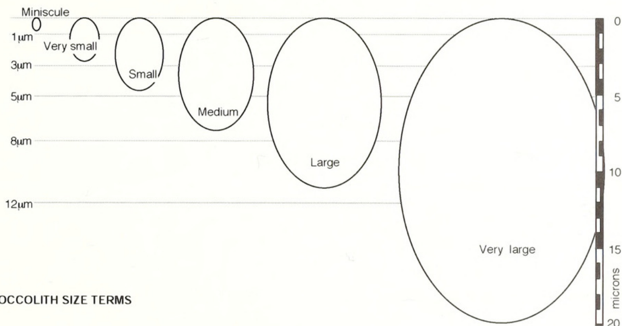
TEXT-FIG. 3. Coccolith sizes and shapes.
