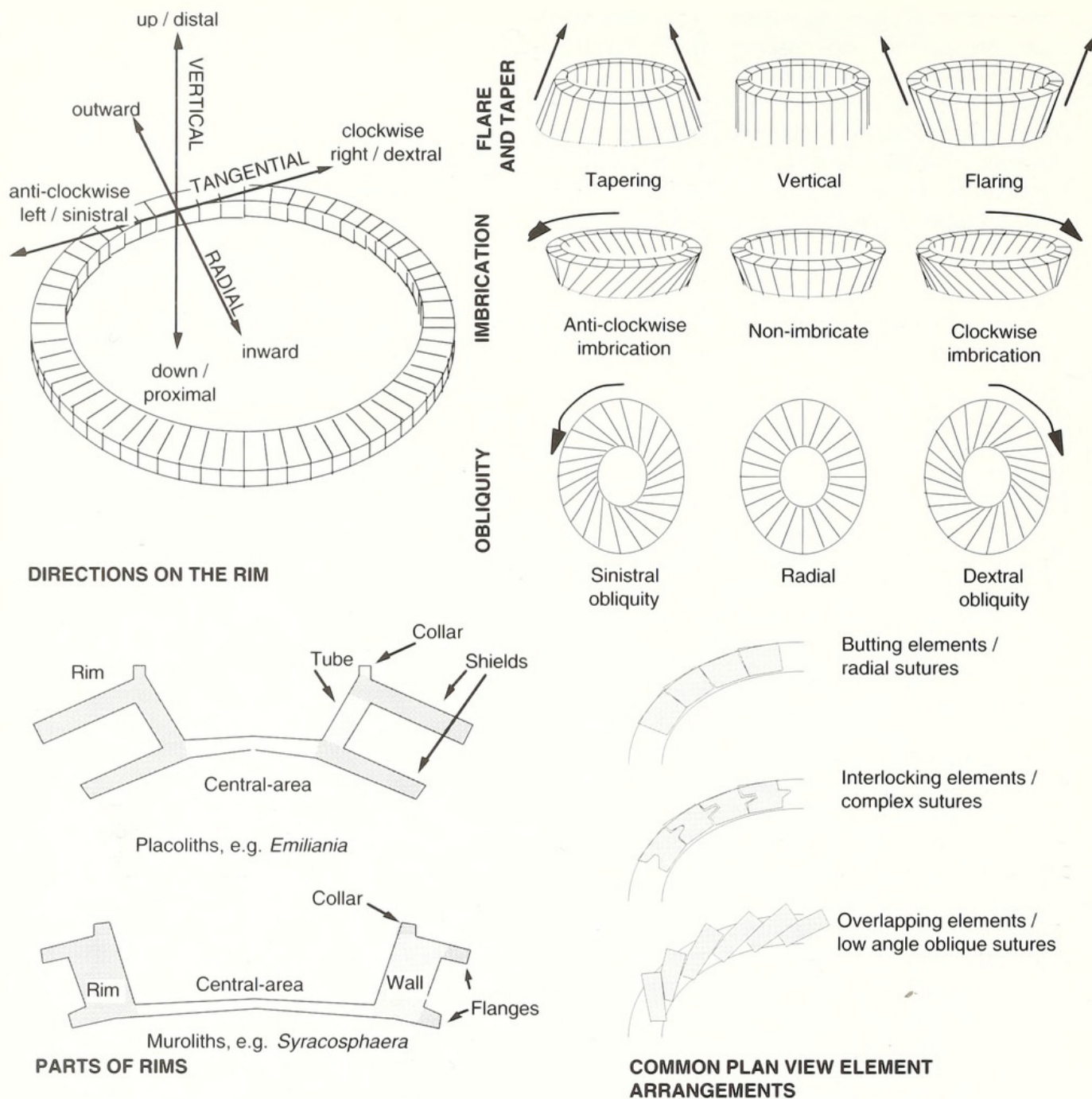
TEXT-FIG. 5. Terms for describing rim structures.
