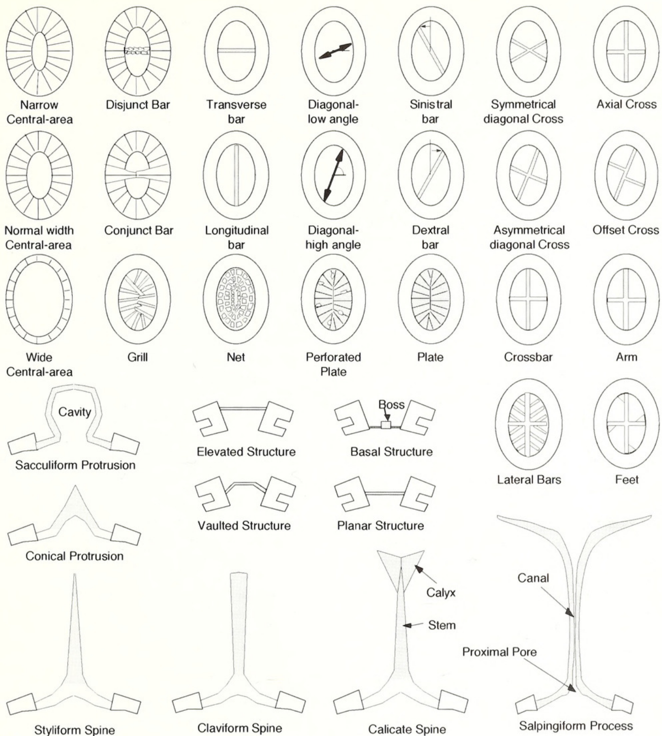
TEXT-FIG. 7. Central area structures.
