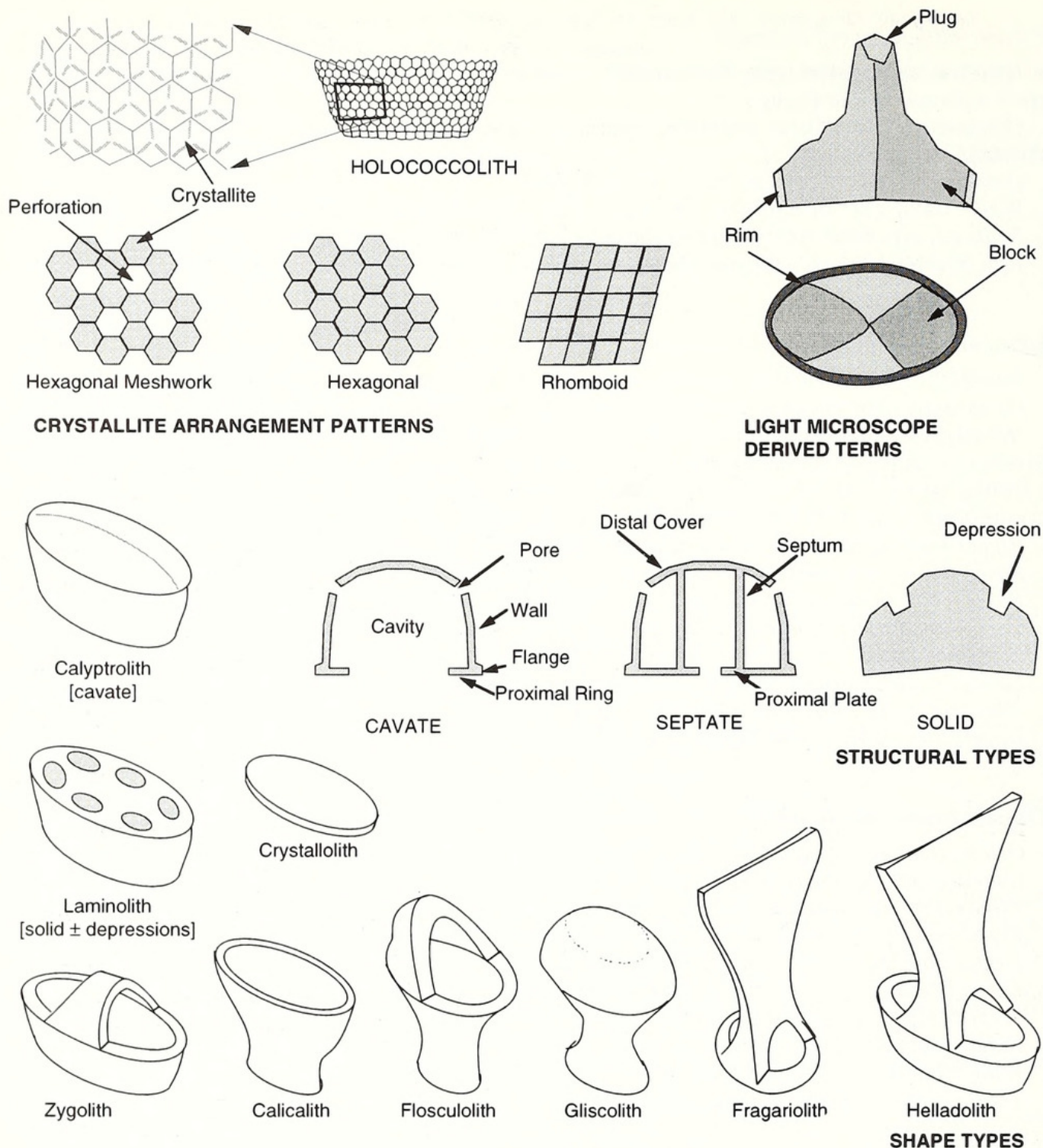
TEXT-FIG. 13. Special terms applied to holococcoliths.
