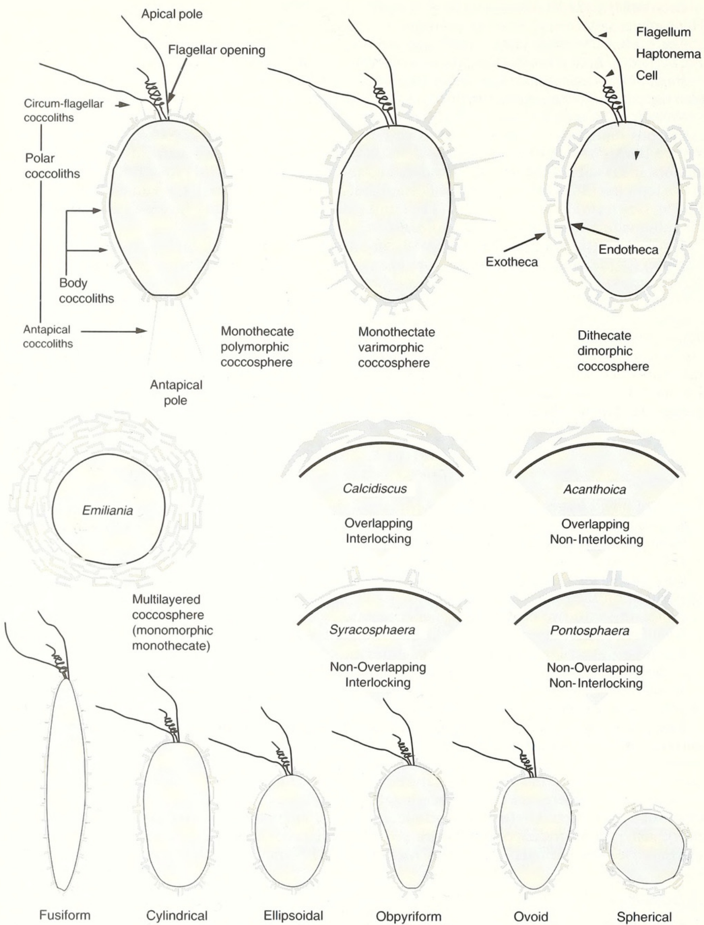
TEXT-FIG. 1. Coccosphere related terms.
