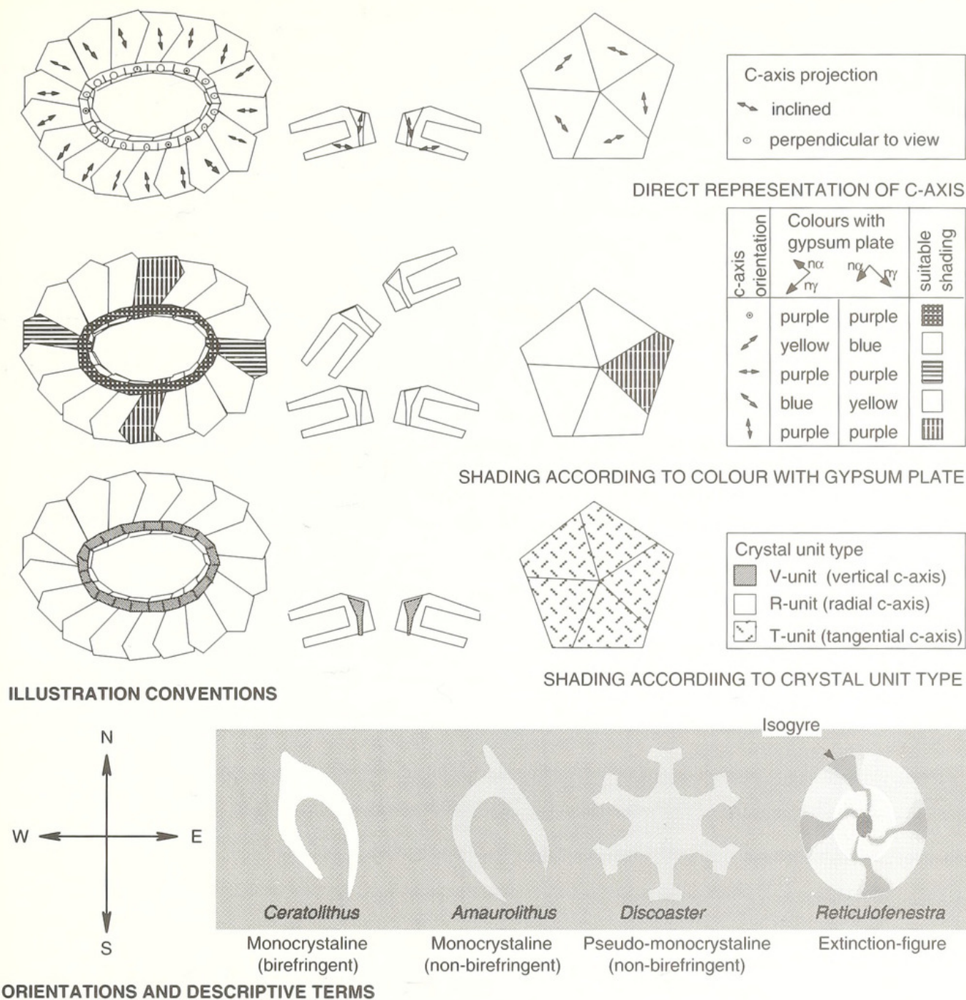
TEXT-FIG. 8. Crystallography: the diagrams showing illustration conventions are based on Watznaueria (plan and side views) and Braarudosphaera ; the figures in the dark box represent the appearance of nannofossils in the light microscope, with cross-polarized light.
