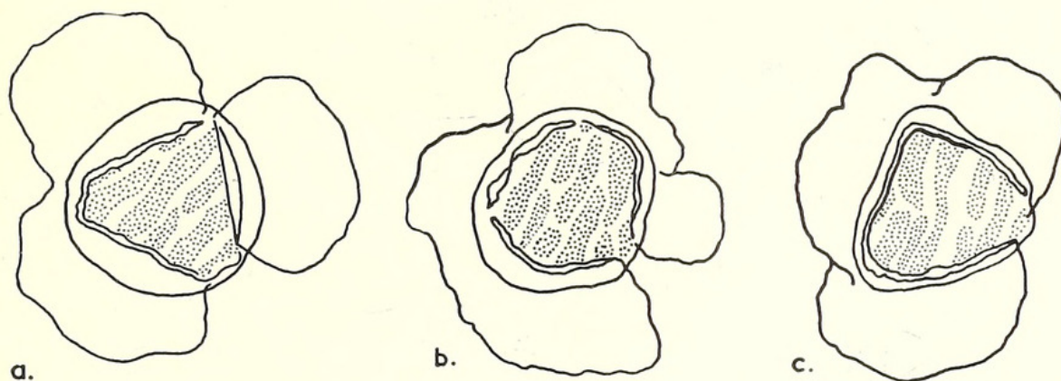
TEXT-FIG. 7. Polar views of Crustaesporites globosus Leschik (drawn from specimens) illustrating variation in the outline of the saccus structure. a , More or less trisaccate condition. b and c , Irregular saccus.
