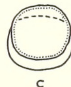
TEXT-FIG. 13. Illinites klausi sp. nov. a , Polar view of proximal face showing the small triradiate mark surrounded by a larger triangular area (based on holotype), \times 1,000 . b and c , Diagrammatic reconstructions. b , Lateral polar section. c , Terminal polar section.
