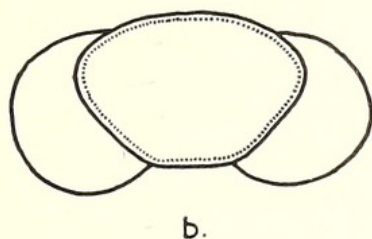
TEXT-FIG. 12. Illinites tectus comb. nov. a , Polar view showing proximal face, on the right, and distal face on the left (drawn from specimen), \times 1,000 . b and c , Diagrammatic reconstructions. b , Lateral polar section. c , Terminal polar section.
