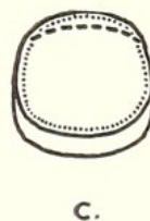
TEXT-FIG. 12. Illinites tectus comb. nov. a , Polar view showing proximal face, on the right, and distal face on the left (drawn from specimen), \times 1,000 . b and c , Diagrammatic reconstructions. b , Lateral polar section. c , Terminal polar section.
