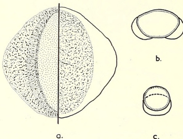
TEXT-FIG. 14. Labiisporites granulatus Leschik. a , Polar view illustrating proximal face with an indistinct monolete mark, on the right, and the distal face on the left (drawn from specimen), \times 1,000 . b and c , Diagrammatic reconstructions. b , Lateral polar section. c , Terminal polar section.
