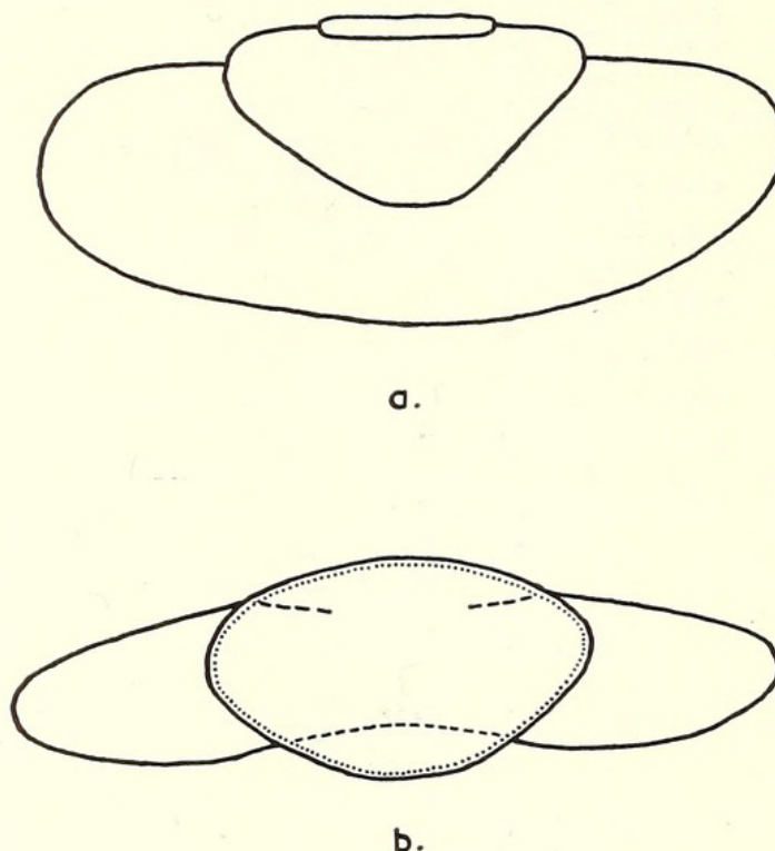
TEXT-FIG. 4. Diagrammatic reconstruction of Potonieisporites Bhardwaj, in lateral (equatorial view). a , The reconstruction of Bhardwaj (1956), showing the saccus unattached (free) over the distal surface. b , The present interpretation where the saccus is attached to the spore body in this region.
