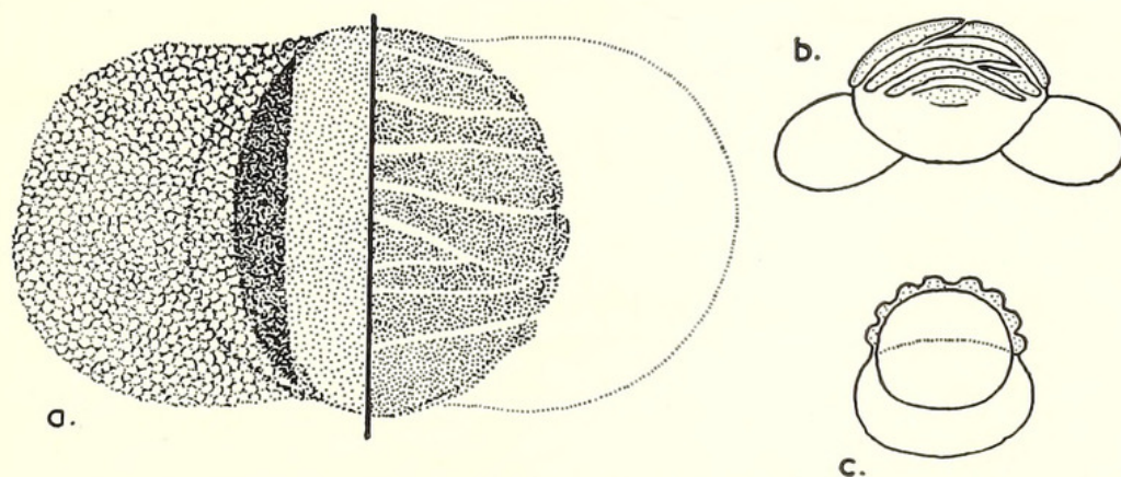
TEXT-FIG. 11. Protohaploxylinus chaloneri sp. nov. a, Showing the form of the proximal taeniae, on the right, and the distal surface on the left-hand side (based on the holotype), \times 1,000 . b and c, Diagrammatic reconstructions. b, Lateral view. c, Terminal polar section.
