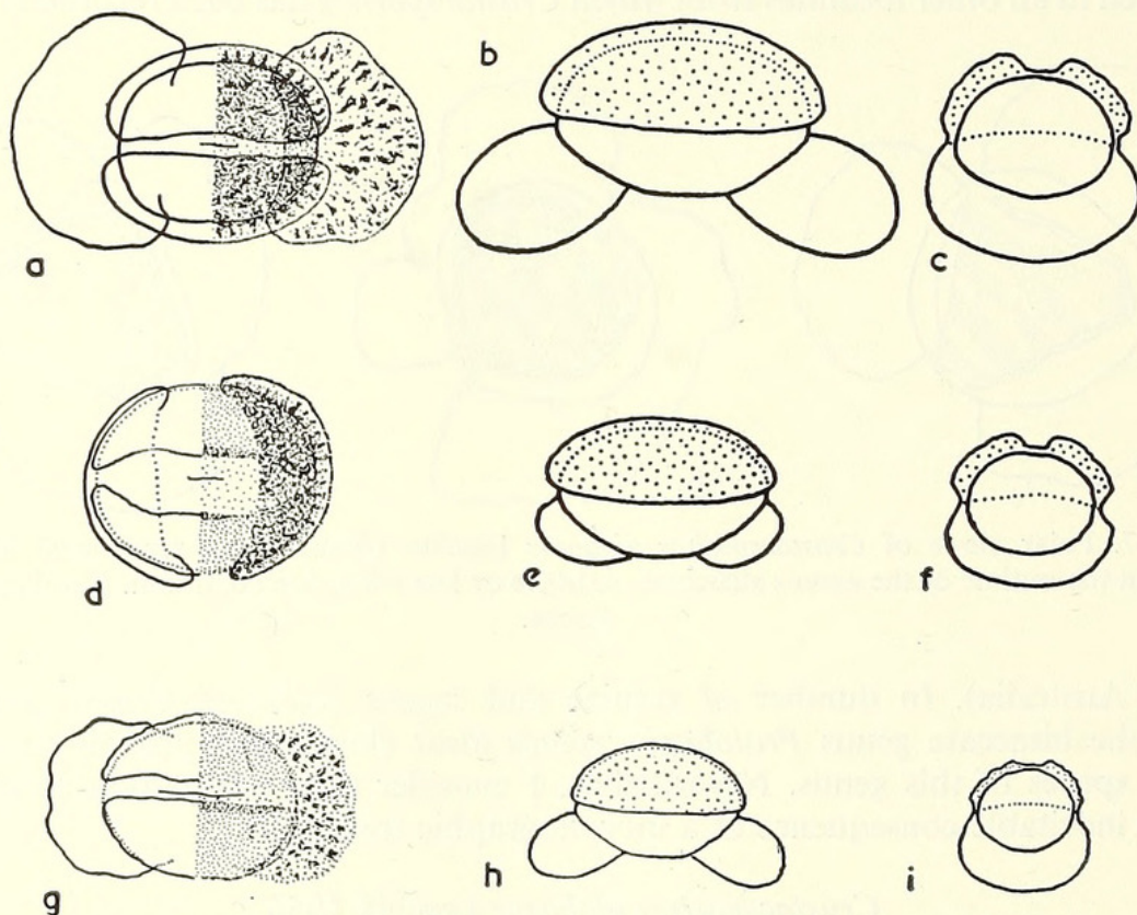
TEXT-FIG. 8. Lueckisporites virkkiae Potonié and Klaus emend. Diagrammatic reconstructions to show the differences between the variants A, B, and C. a-c , Variant A. d-f , Variant B. g-i , Variant C. a, d, g , Proximal polar views. b, e, h , Lateral views. c, f, i , Terminal polar sections.
