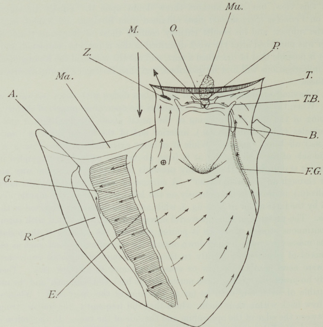
TEXT-FIG. 5.— Vermetus novae hollandiae ; mantle cavity exposed by cutting of the mantle along the right-hand side. \times 2\frac{1}{4} . A., anus; B., buccal mass; E., endostyle; F.G., food groove; G., gills; M., mouth; Ma., mantle; Mu., mucus from pedal gland; O., operculum; P., aperture of pedal gland; R., rectum; T., pedal tentacle; T.B., tentacle on buccal mass; ⊕, beginning of rejection currents for heavy material; Z., site of accumulation of waste matter. Small arrows indicate direction of ciliary currents, large vertical arrow position of inhalent current.
