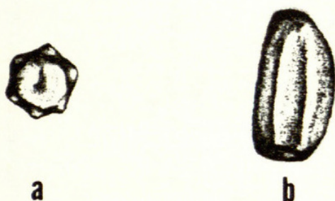
FIG. 1.—Sketch of a typical wood-dwelling termite fecal pellet, enlarged approximately 18x normal size. Cross-sectional view (a) reveals hexagonal shape, while parallel ridges are evident on longitudinal view (b).
