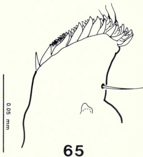
FIGS. 62–65. Eumicrota cornuta Casey, larval instar III. 62 , Labrum, adoral aspect (epipharynx); 63 , labium, ventral aspect; 64 , mala of maxilla, ventral aspect; 65 , mala of maxilla, dorsal aspect.
