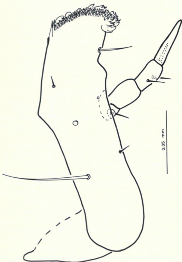
FIGS. 5-8. Agaricochara laevicollis Kraatz, larval instar III. 5, Labrum, dorsal aspect; 6, labrum, adoral aspect (epipharynx); 7, maxilla, ventral aspect; 8, mala of maxilla, dorsal aspect.
