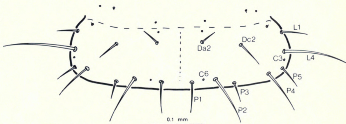
FIGS. 54–56. Eumicrota corruscula (Erichson), larval instar III. 54, Proleg, anterior aspect; 55, pronotum; 56, mesonotum.
