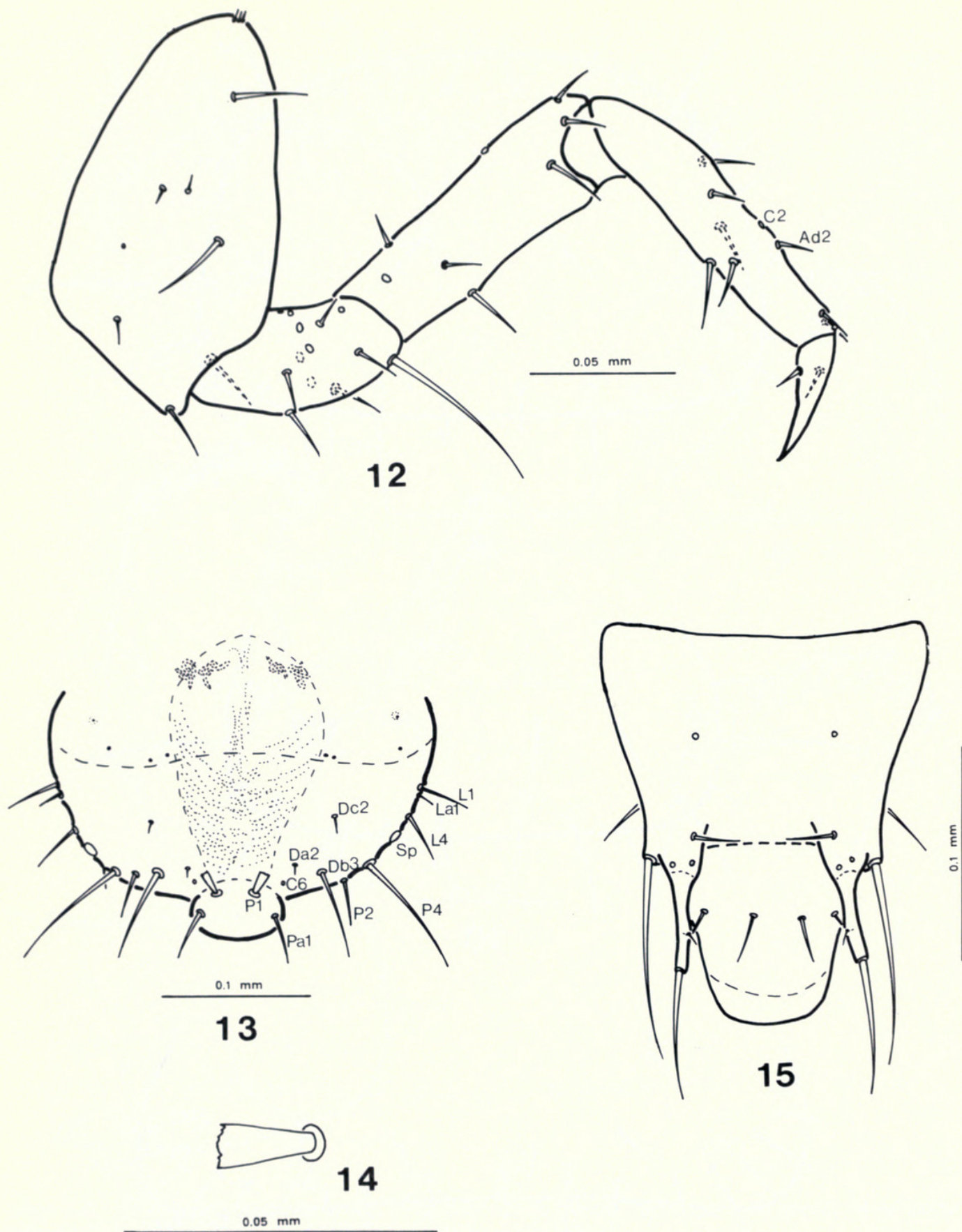
FIGS. 12-15. Agaricochara laevis Kraatz, larval instar III. 12, Proleg, anterior aspect; 13, abdominal tergum VIII; 14, brushlike seta, P1 of abdominal tergum VIII, detail; 15, abdominal terga IX-X.
