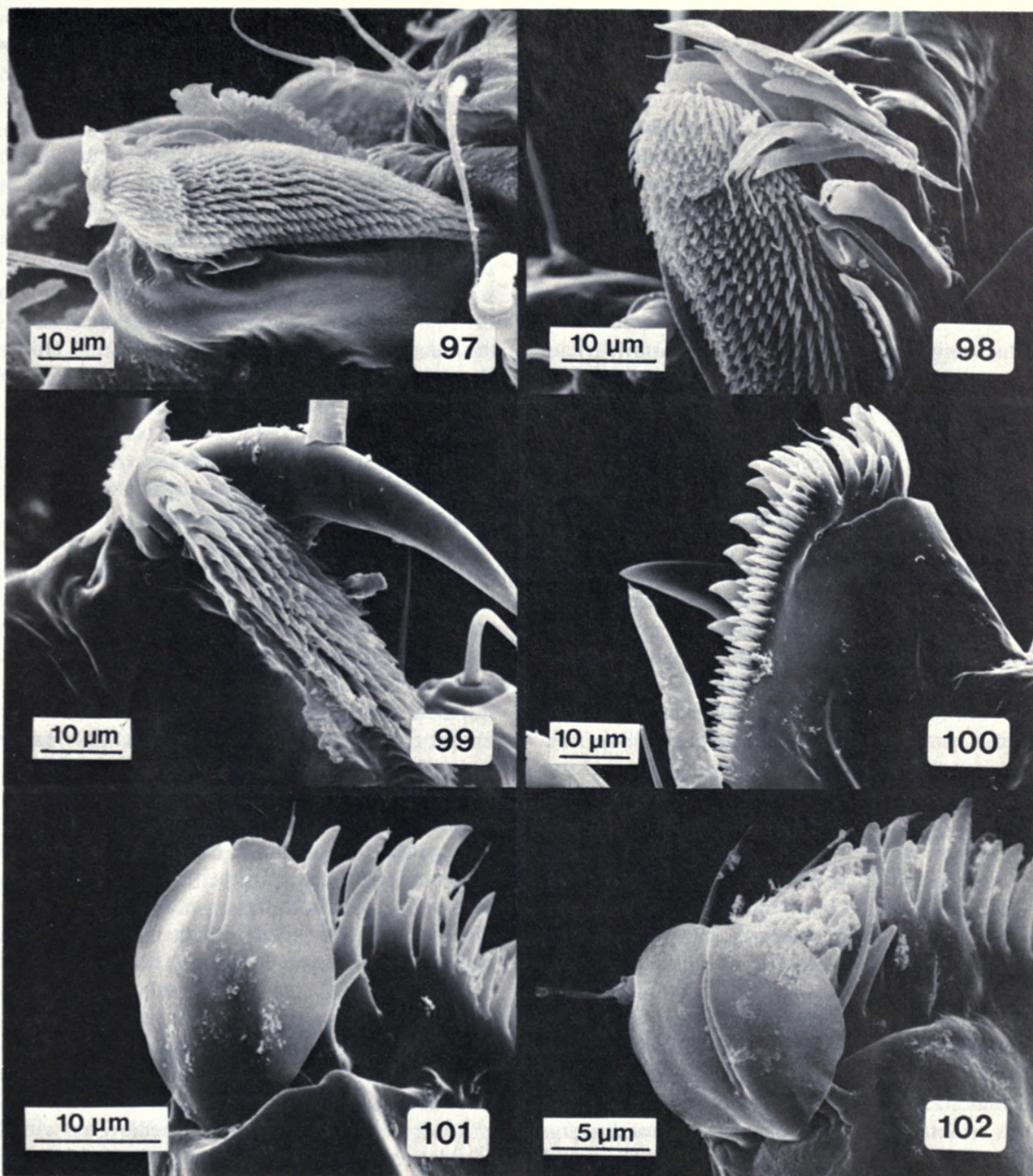
FIGS. 97–102. SEM micrographs of maxillae of larval instar III Gyrophaenina. 97 , Brachychara sp. 2, apex of mala; 98 , Brachychara sp. 1, apex of mala; 99 , Agaricomorpha apacheana (SeEVERS), apex of mala; 100 , Gyrophaena nana (Paykull), apex of mala; 101 , Gyrophaena nana (Paykull), outer apical aspect of mala showing emarginate foliose scale; 102 , Eumicrota corruscata (Erichson), outer apical aspect of mala showing emarginate foliose scale.
