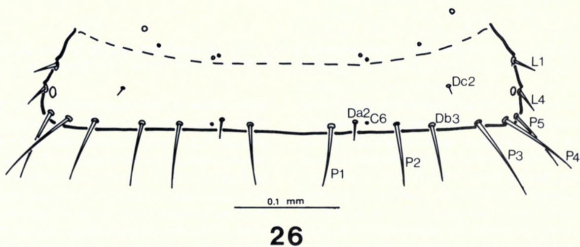
FIGS. 24–26. Agaricomorpha apacheana (Seevers), larval instar III. 24 , Pronotum; 25 , mesonotum; 26 , abdominal tergum I.
