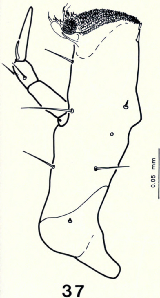
FIGS. 35–38. Brachychara species 1, larval instar III. 35, Labrum, adoral aspect (epipharynx); 36, labrum, dorsal aspect; 37, maxilla, ventral aspect; 38, mala of maxilla, detail, dorsal aspect.
