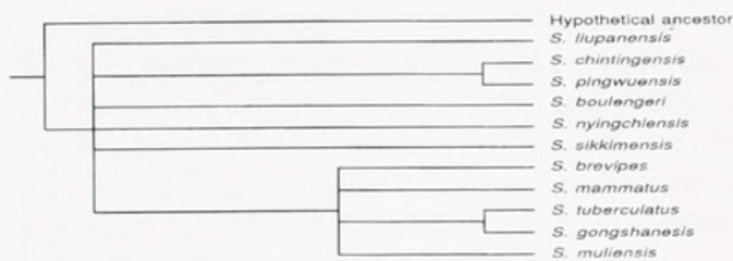
Figure 2. Strict consensus tree of the phylogeny of Scutiger , derived from our reanalysis of Ye et al.'s (1992) original data.
