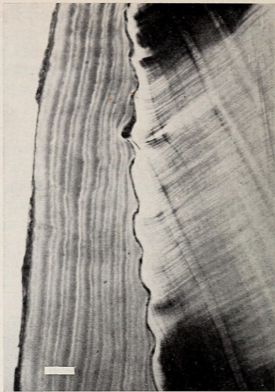
Fig. 8. Thin ground longitudinal section of mandibular tooth of a sperm whale. There are 36 incremental layers in dentine and cementum, not all of which are shown. Cementum to left of picture; transmitted light (bar = 1 mm.)
