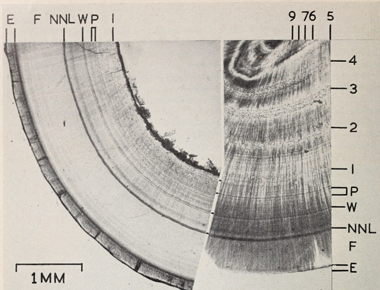
Fig. 3. Left, thin ground section of canine tooth of a 1-year-old male crabeater seal. Right, section of canine of 9-year-old female; transmitted light. (E — enamel, F — foetal dentine, NNL — neonatal line, W — weaning, P — position of inner border of dentine in 6-month-old pups, 1-9 = annual rings)
