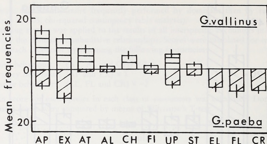
Fig. 4. Mean frequencies ( \pm S.E.) of agonistic behaviours in G. vallinus - G. paeba encounters ( n = 9 )
