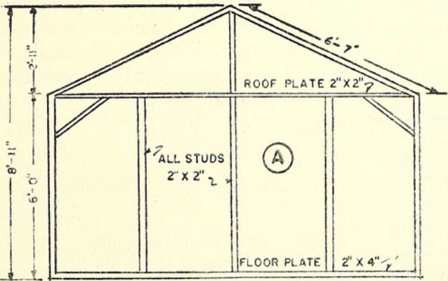
END VIEW
