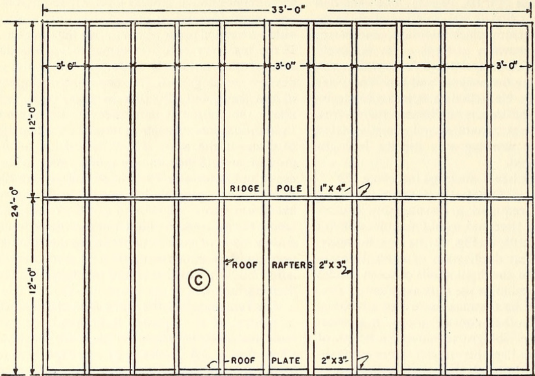
TOP VIEW
